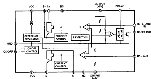
IC201 : M5290P Constant-Voltage Tracking Supply with Reset
