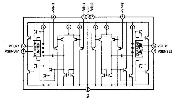
IC304 : LA6510 Dual Power Operational Amp
