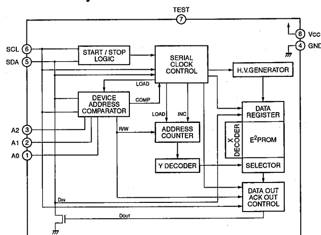
IC320 : S-24C01ADP Electrically Erasable PROM
