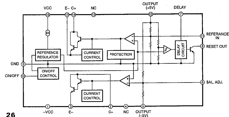
IC201 : M5290P Constant-Voltage Tracking Supply with Reset
