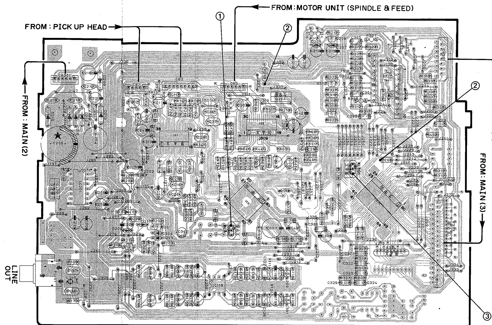
P. C. B. MAIN ( 1 )
