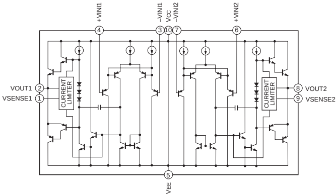
IC401 : LA6510 Dual Power Operational Amp
