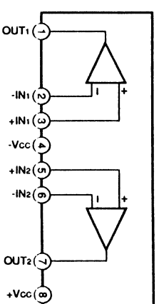
IC35 : BA15218N or M5218AL Dual OP-Amp
