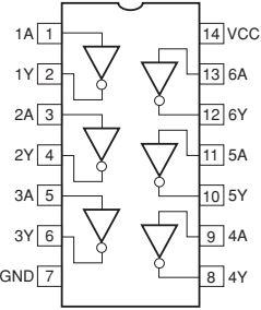
IC802: TC74HCU04AFEL Hex Inverters
