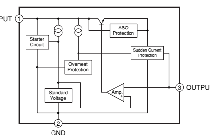
IC702: M5237L Regulator
