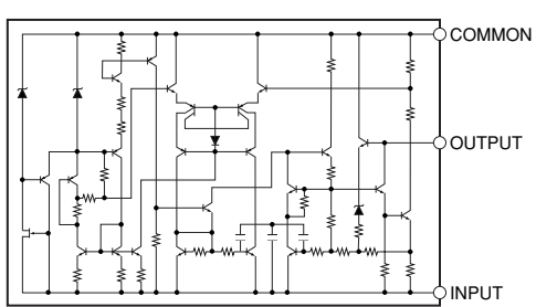
IC703: NJM79M05FA Voltage Regulator
