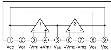
IC500: \mu PC4570HA Dual OP-Amp
