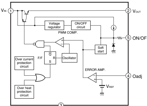
IC700-701: PQ1CG2032FZ Voltage Regulator
