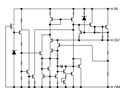
IC603: NJM78M05FA 3-terminal positive voltage regulator
