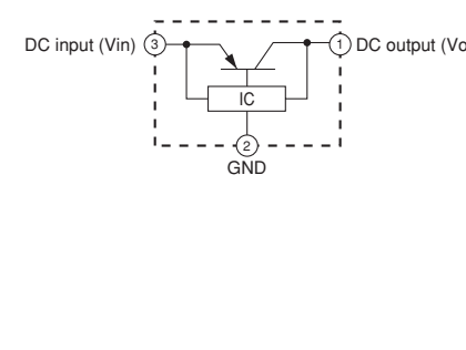
IC605: PQ033ES3MXP Low power loss regulator
