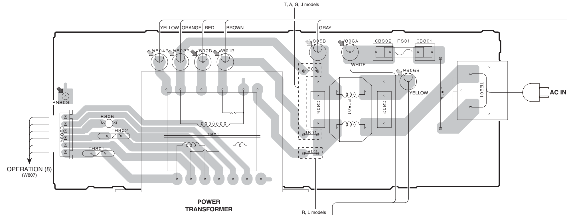
OPERATION (5) P.C.B. (Side A)
