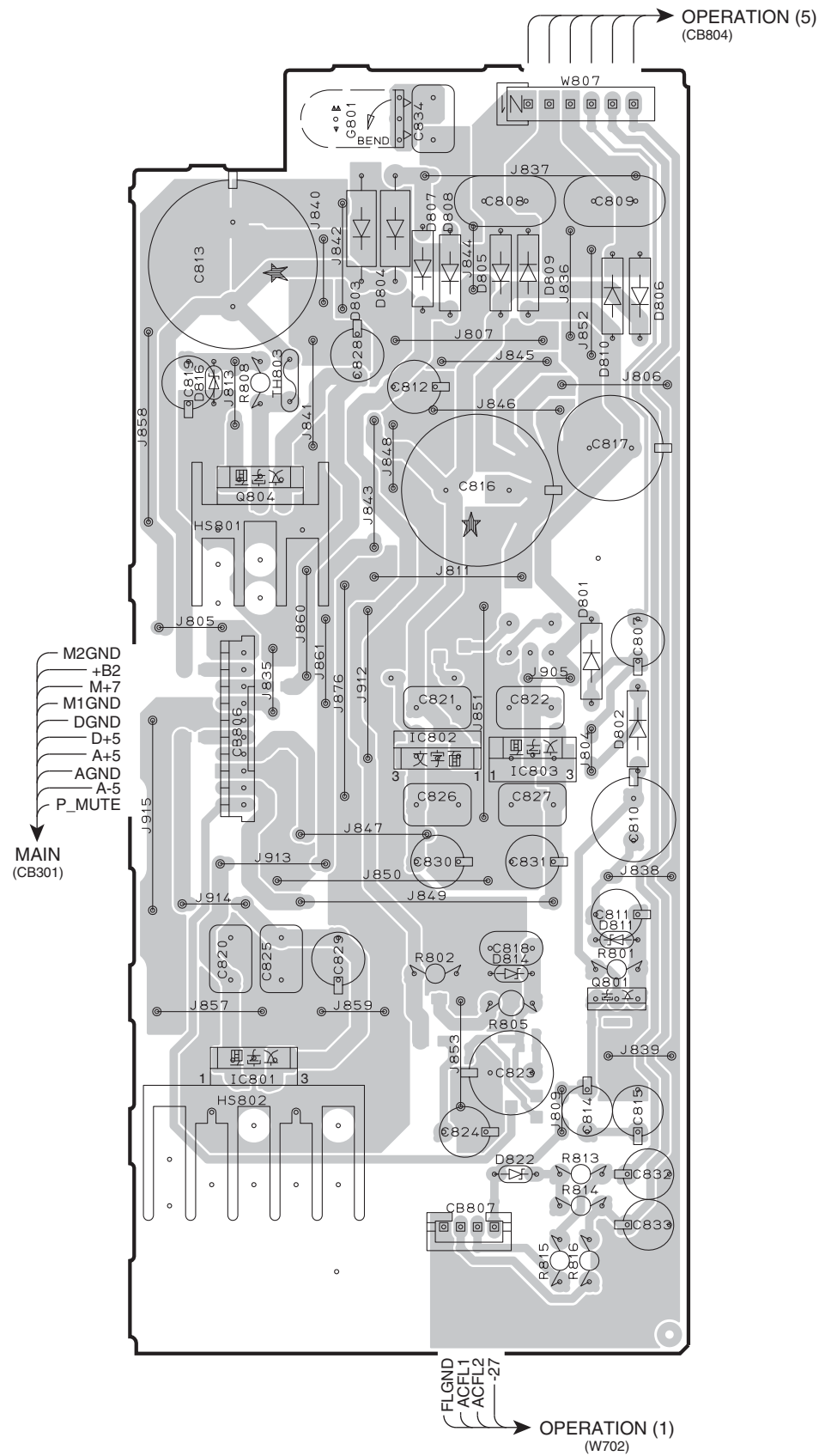
OPERATION (8) P.C.B. (Side A)
