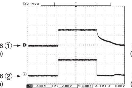
POINT D ①/ IC306 (2 pin), ②/ CB306 (1 pin)
