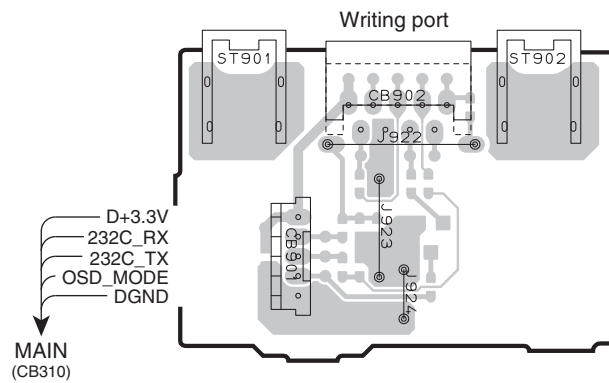
OPERATION (9) P.C.B. (Side A)
