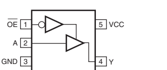
IC406: SN74LVC1G125DCKR Single bus buffer gate
