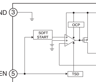
IC409: BD00GA3WEFJ-E2 300 mA variable output LDO regulator
