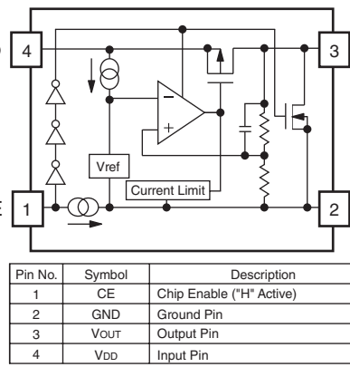
IC408: RP130Q331D-TR-F Voltage regulator
