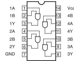
IC910: TC74VHCT08AFT Quad 2-input AND gate
