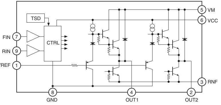
IC418, 419: BA6956AN Reversible motor driver
