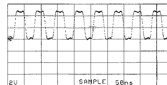
Point ② (Pin 59 of IC11) V: 2V/div H: 50nsec/div DC range 1:1 probe
