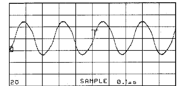
Point ③ (Pin 31 of IC12) V: 2V/div H: 0.1 \mu sec/div DC range 1:1 probe
