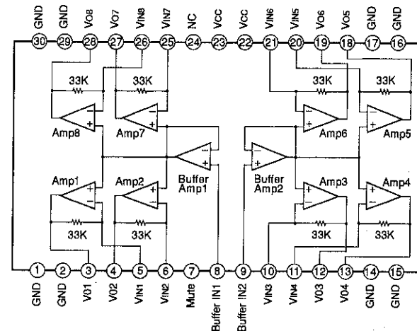
IC6 : LA6536M 4 Channel BTL Driver
