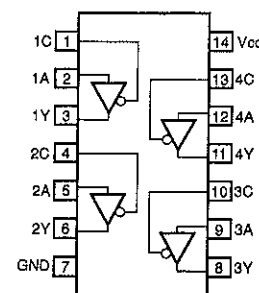
IC16 : TC74HC125AP Quad 3 State Bus Buffers
