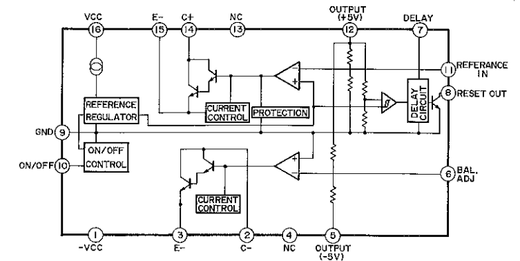
IC27 : M5290P Constant-Voltage Tracking Supply with Reset
