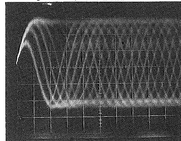
Point ① TP1 (EFM) V: 0.2V/div H: 0.5 \mu sec/div AC range 1:1 probe
