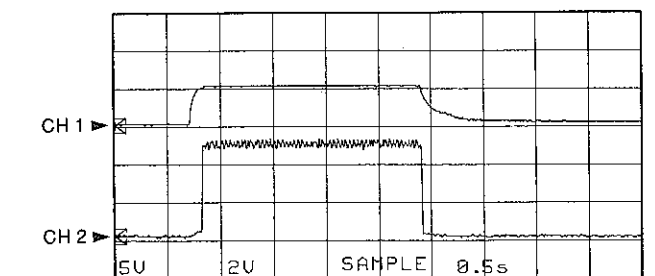
Point ④ (CH 1: Collector of Q9) (CH 2: Pin 8 of IC27) V: 5V/div ... CH1 V: 2V/div ... CH2 H: 0.5sec/div DC range 1:1 probe
