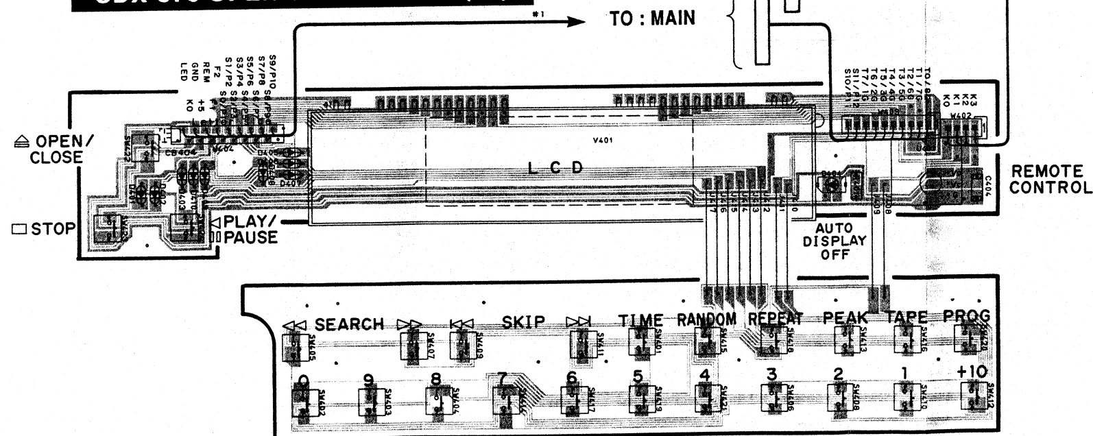
CDX-670 OPERATION P. C. B. ( 2 )
