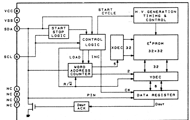
IC9 : M5290P
