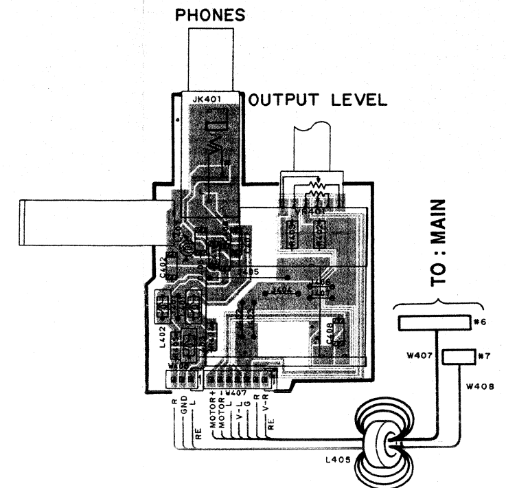
CDX-870/670 OPERATION P. C. B. ( 3 )
