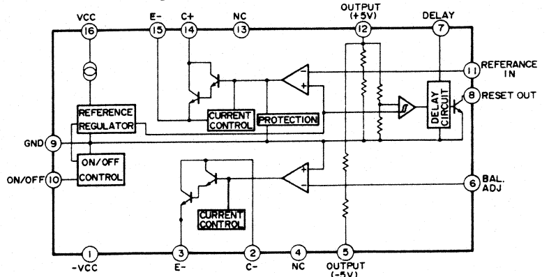
IC9 : M5290P
