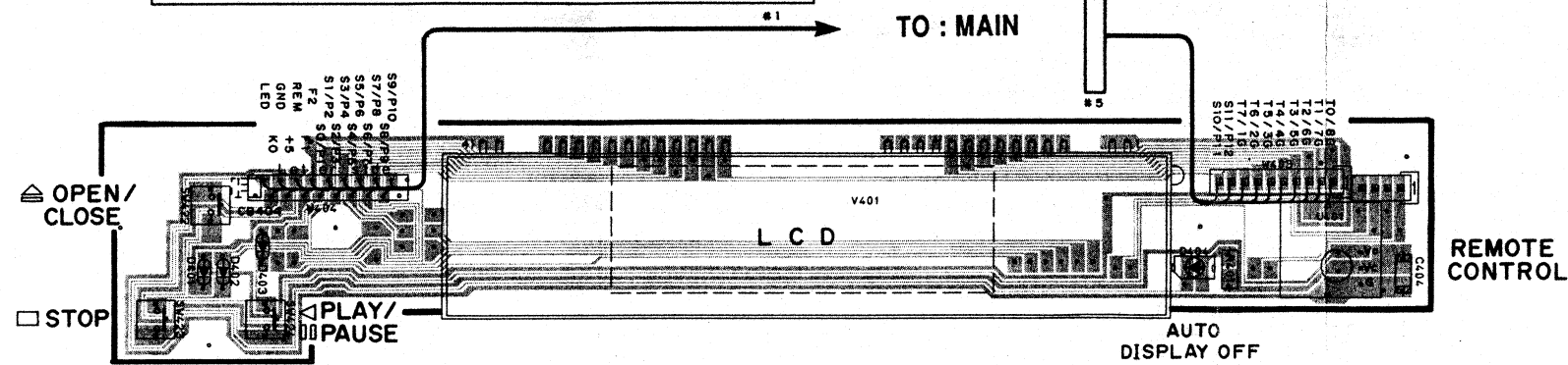
CDX-870 OPERATION P. C. B. ( 2 )
