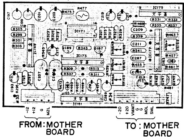
UNIT AMP (12)
