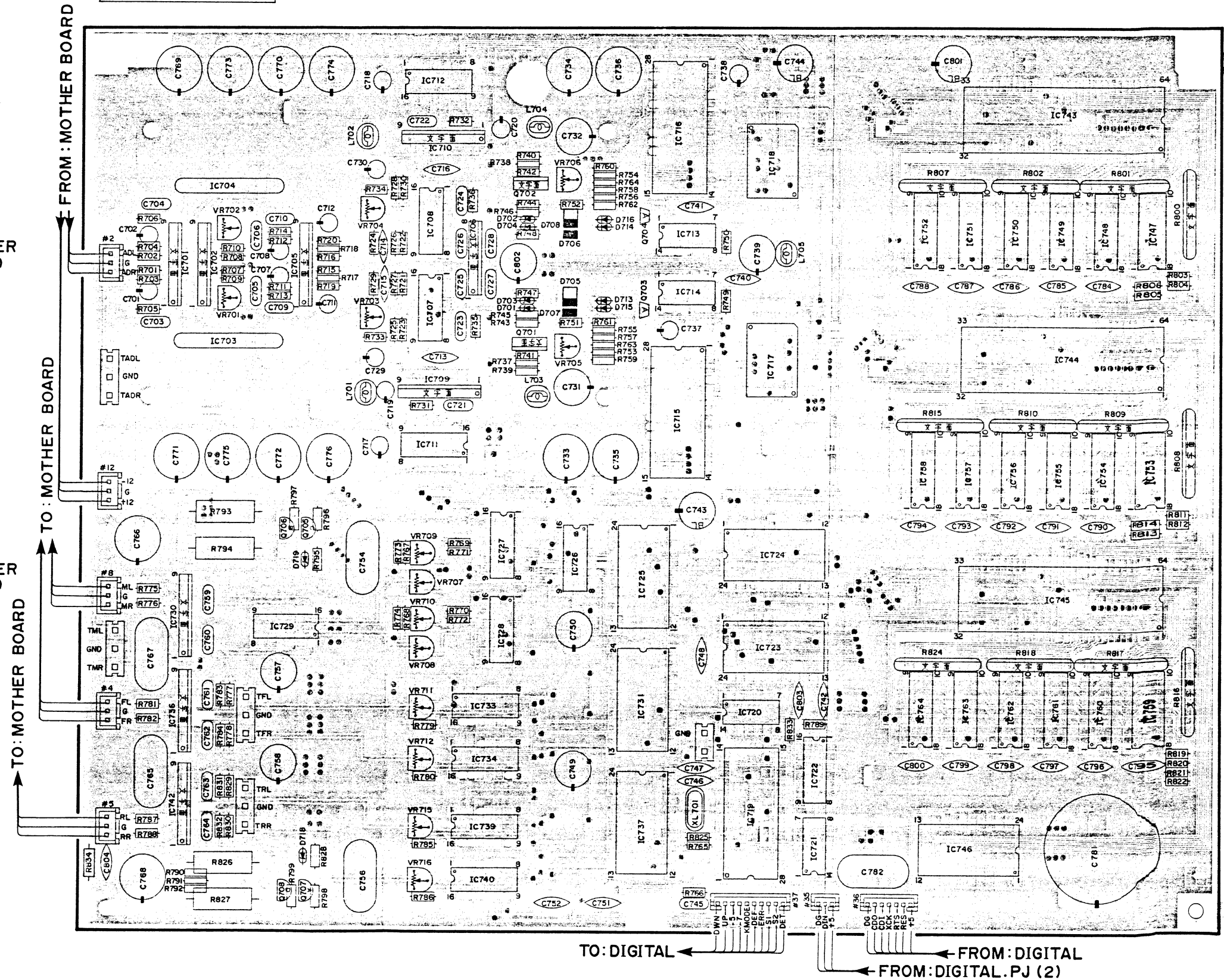
DSP Circuit Board
