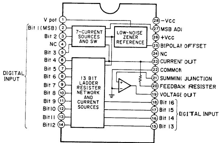
IC715, 716: PCM54HP D/A Converter
