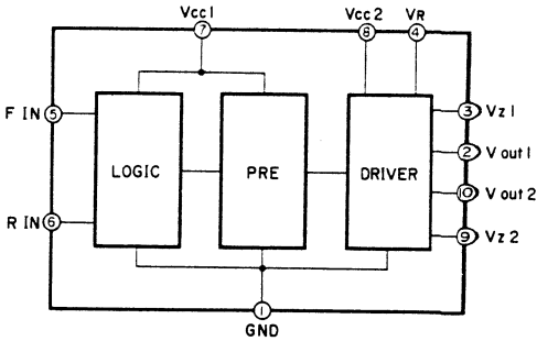
IC8g: BA6209 Motor Driver
