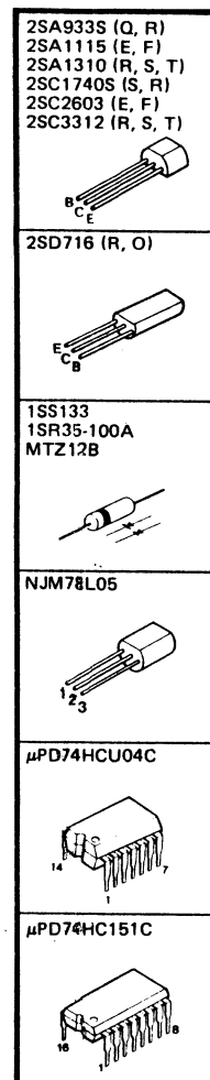
PIN CONNECTION DIAGRAM OF TRANSISTORS, DIODES AND ICS.
