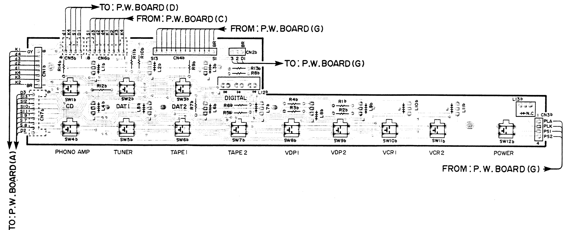
PW Circuit Board (B)
