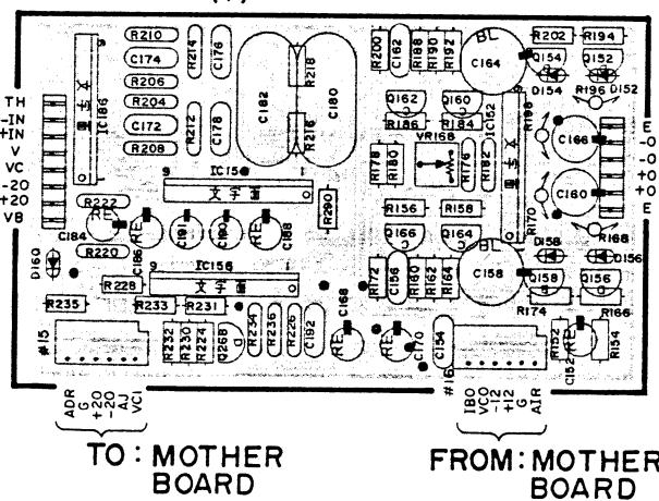
UNIT AMP (1)
