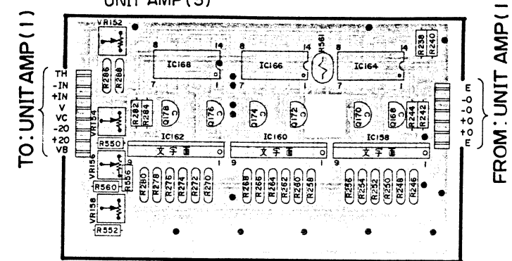
UNIT AMP (3)
