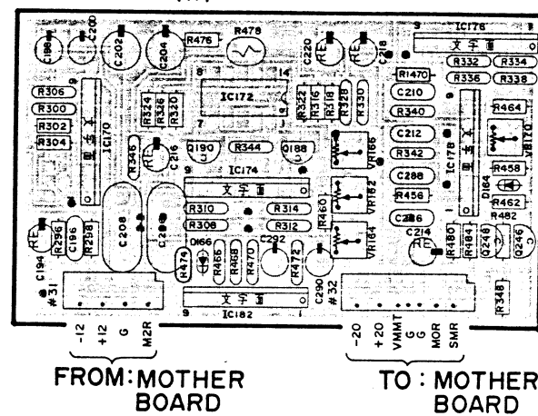
UNIT AMP (11)
