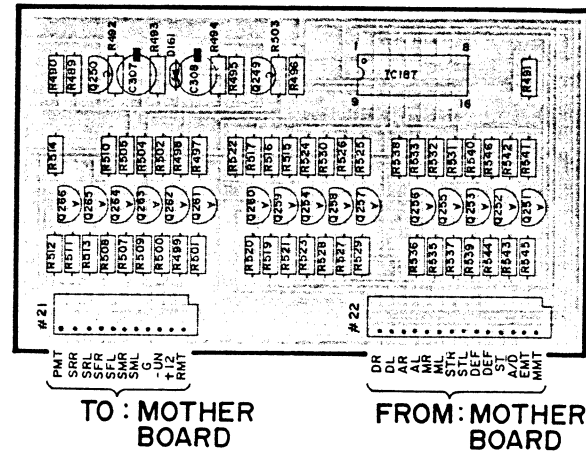
UNIT AMP (4)
