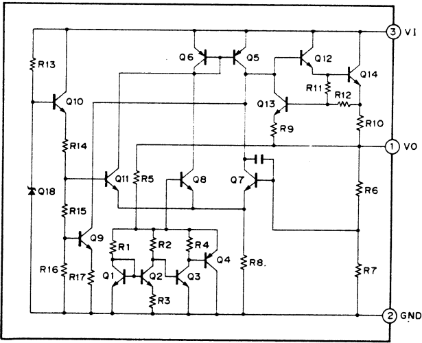
IC951: NJM78L05 Regulator
