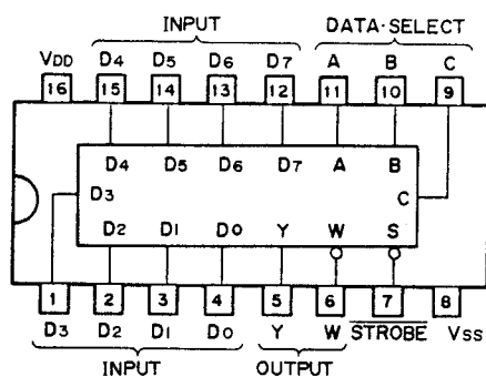
IC908 ~ 910: \mu PD74HC151C 8 to 1 Data Selector
