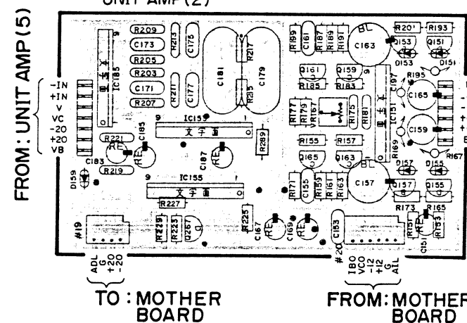
UNIT AMP (2)
