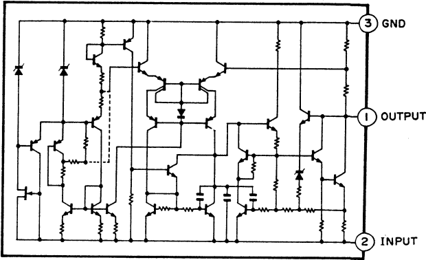
IC602: NJM79M05A Regulator
