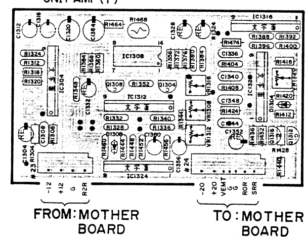
UNIT AMP (7)
