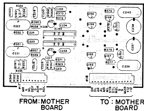
UNIT AMP (4)
