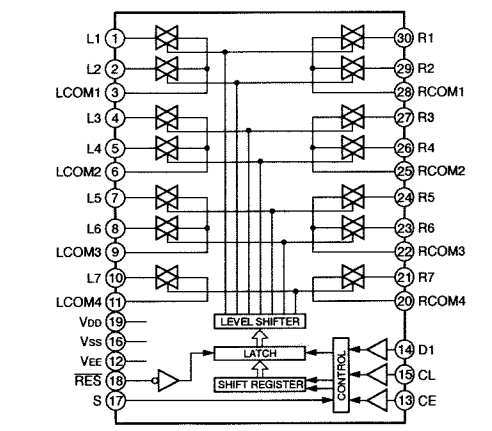
IC308, 310 : TC9299P Electric Controlled Volume
