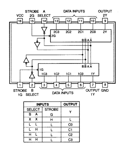
IC320 : TC74HC153AP Dual 4 to 1 Data Selectors
