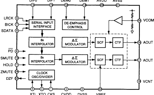
IC10-12 : AK4320 1 bit D/A Converter
