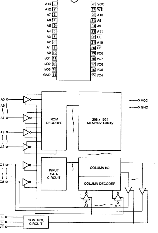
IC8 : LH5P832N-10 256K Pseudo Static RAM
