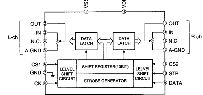
IC309 : LC7535 Electric Controlled Volume
