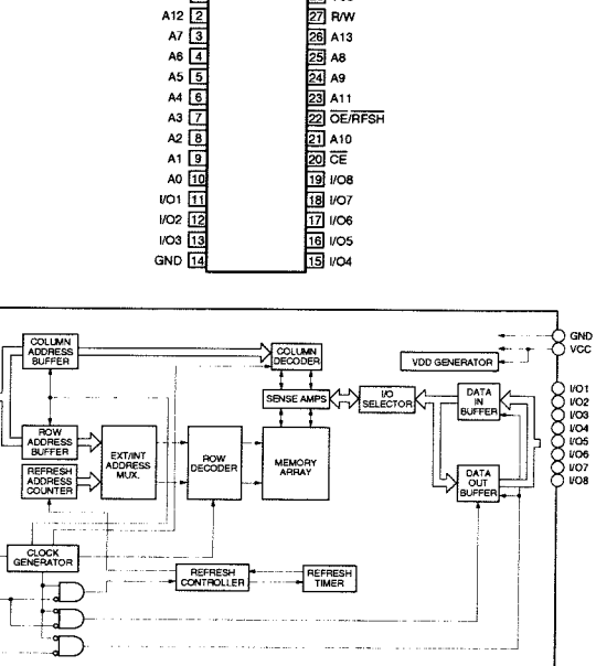
IC8 : LH5P832N-10 256K Pseudo Static RAM
