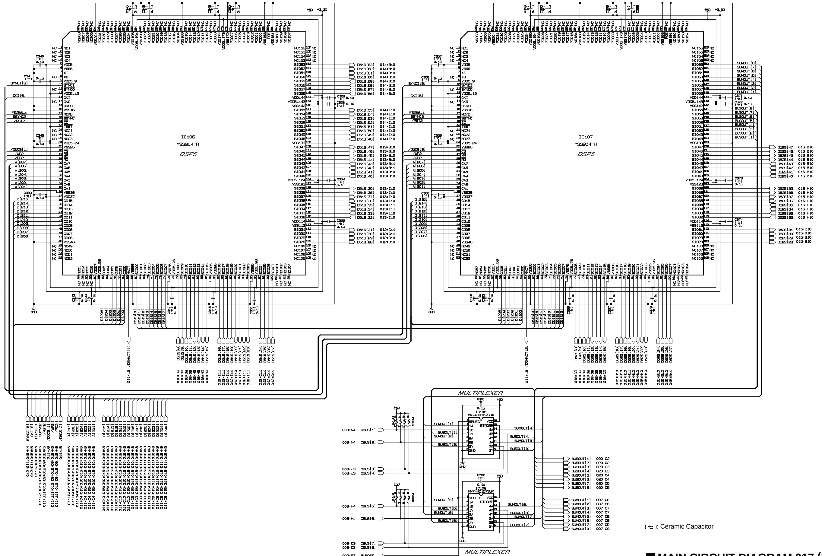
MAIN CIRCUIT DIAGRAM 017 (DME32)
