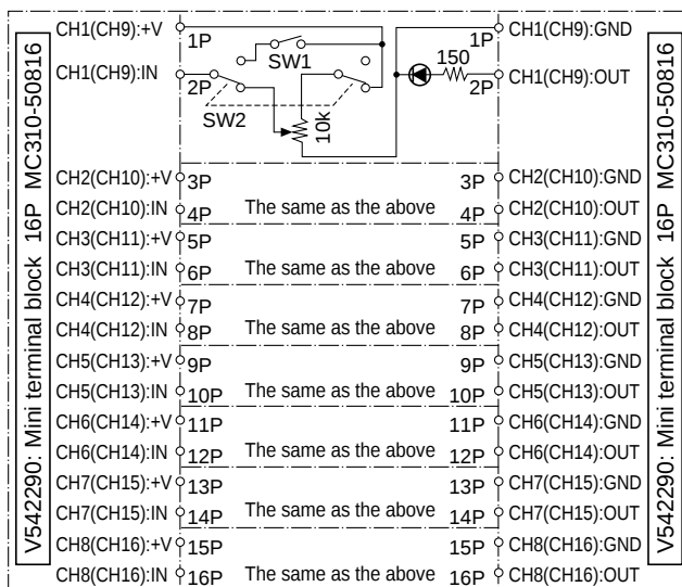
Circuit diagram for GPI inspection jig
