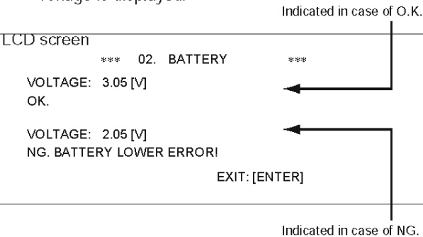
Fig. 13. BATTERY Test Screen
