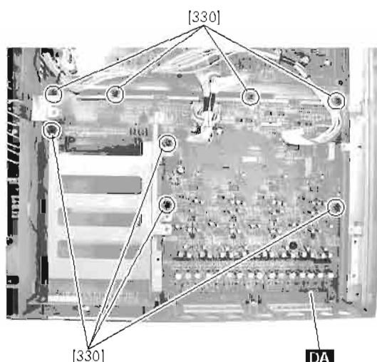
[330]: Bind Head Tapping Screw-B (+バインドB タイト) 3.0X6 MFZN2BL (EP600230)
