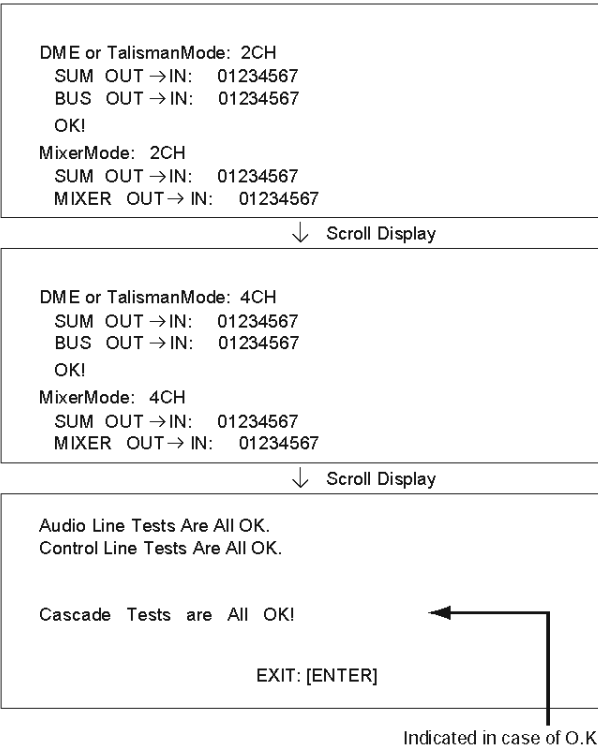
Fig. 35. CASCADE Test Screen (1)
