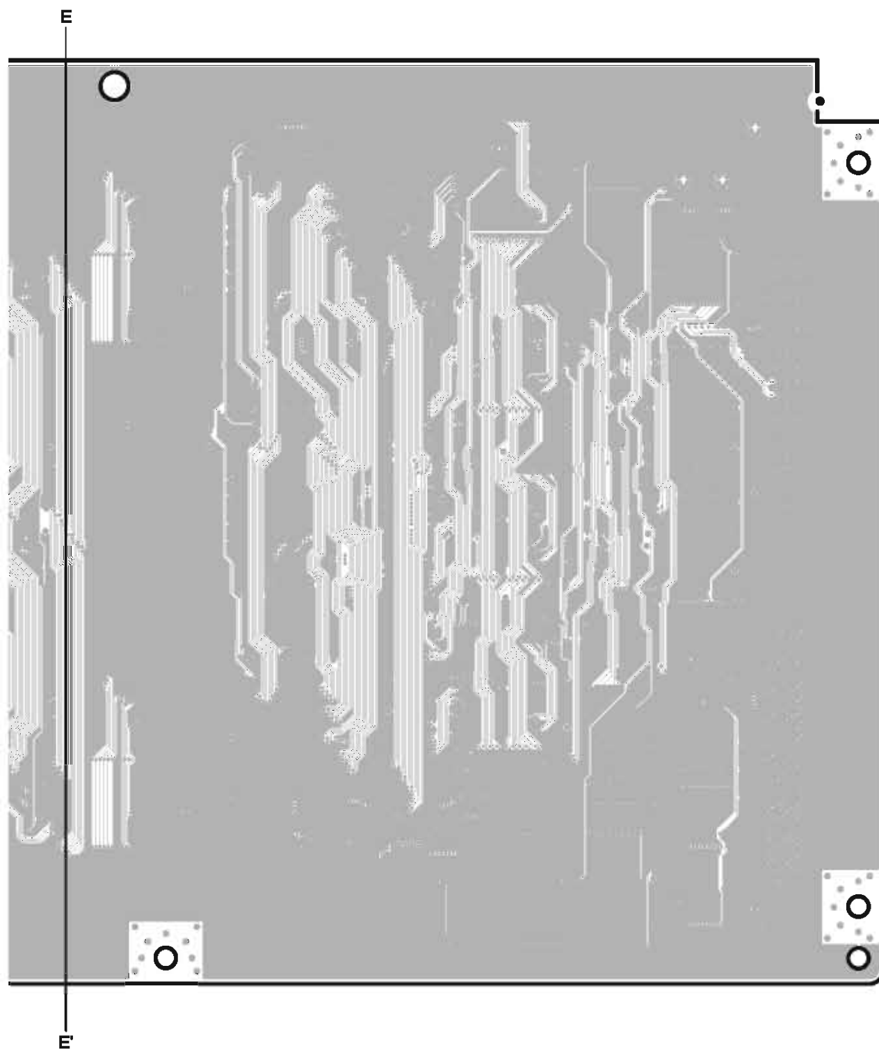
Component side (部品側) 3 layer (3層)
