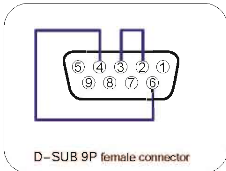
Fig. 3. COM Terminal Connection Jig for RS232C/422 Loop Back Test
