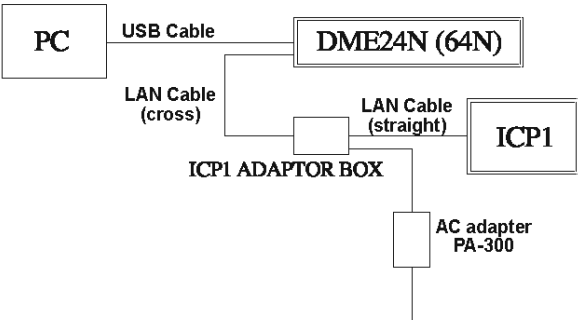
Fig. 1. Connection with PC
