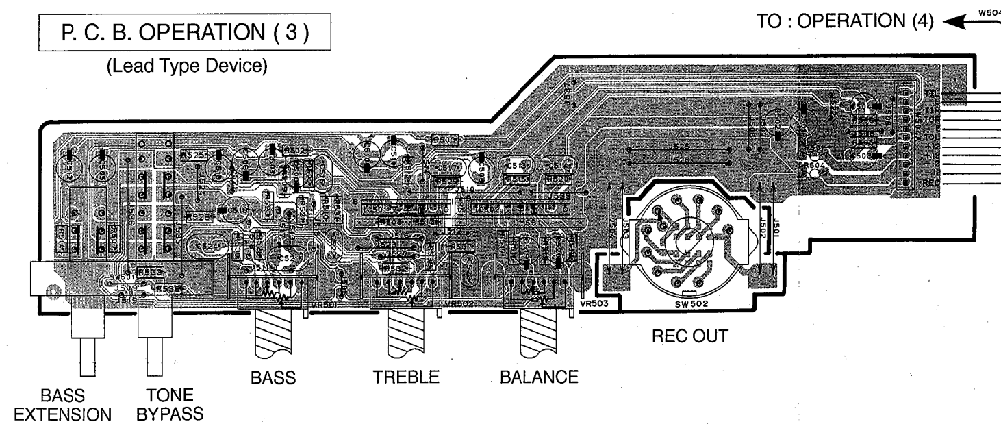
P. C. B. OPERATION ( 3 )
