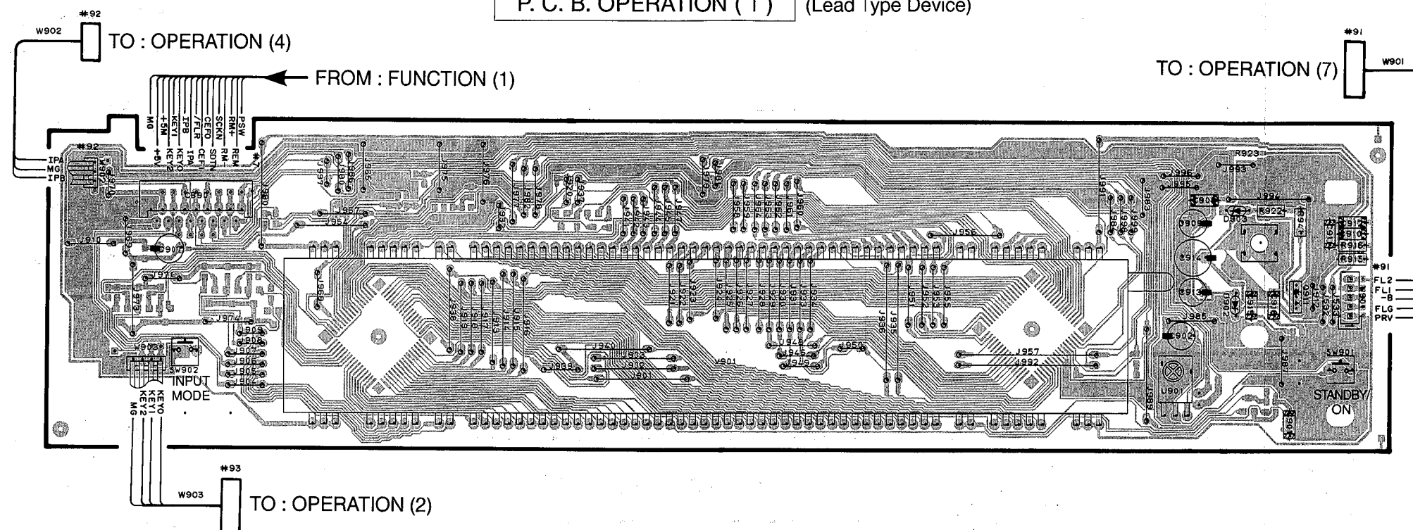
P. C. B. OPERATION ( 1 ) (Lead Type Device)
