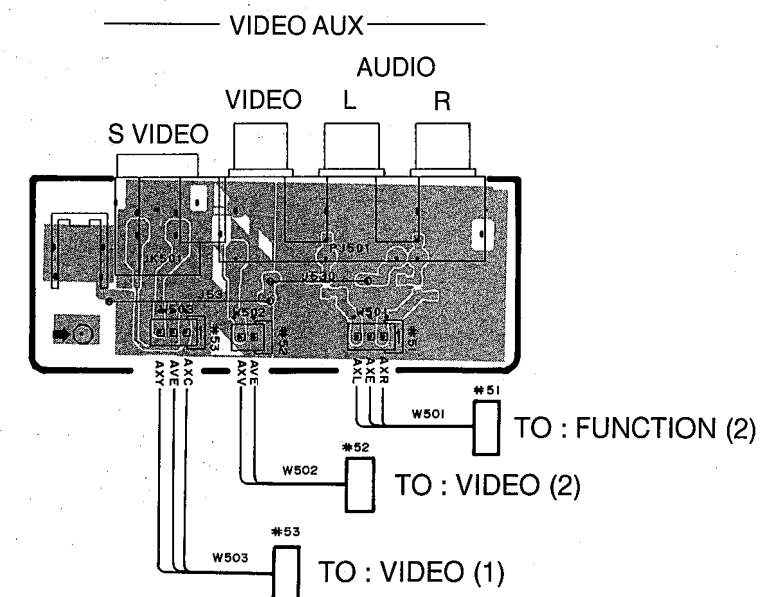
P. C. B. OPERATION ( 5 )
