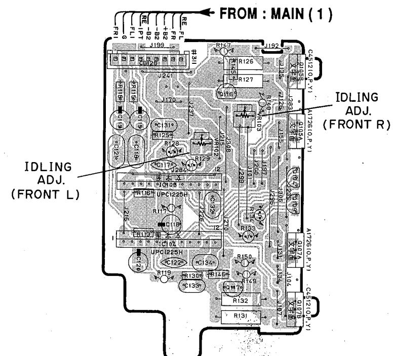
EFFECT P. C. B. ( 3 )
