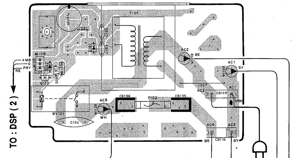
EFFECT P. C. B. ( 7 )
