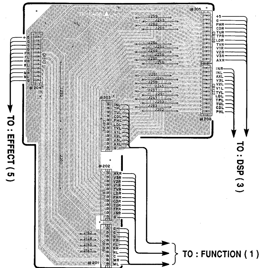
EFFECT P. C. B. ( 1 )
