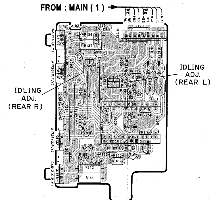
EFFECT P. C. B. ( 4 )
