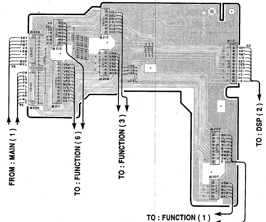
EFFECT P. C. B. ( 2 )
