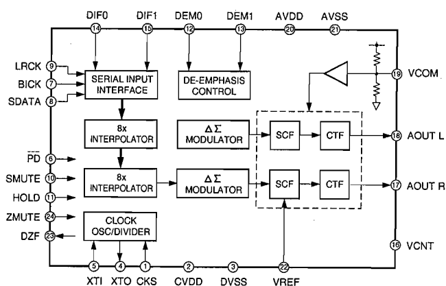
IC25~28 : AK4320-VM 1 bit D/A Converter
