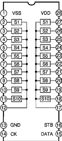
IC403, 405 : TC9273N-004 Analog Function Switch
