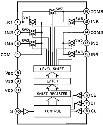
IC8 : LC7824 Analog Function Switch
