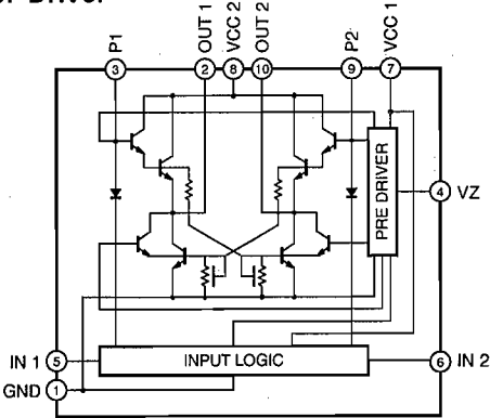
IC301, 302 : LB1641 Motor Driver
