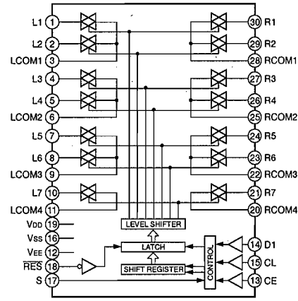
IC20 : LC78213 Analog Function Switch
