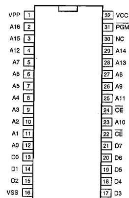
IC44 : MSM27C131ZB 131,072-word x 8 bit One Time PROM
