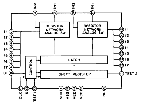
Graphic Equalizer
