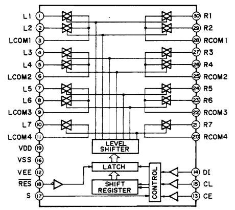
Analog Function Switch
