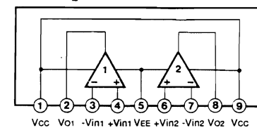
IC104~106, 111, 116 : \mu PC4570HA Dual OP-Amp
