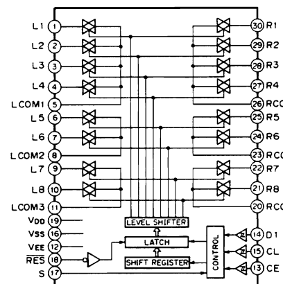
Analog Function Switch
