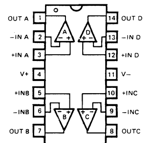
IC109, 113 : \mu PC4574C 4-Channel OP-Amp
