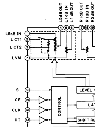
Electric Controlled Volume
