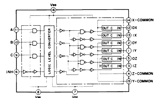
Triple 2-Channel Multiplexer/Demultiplexer
