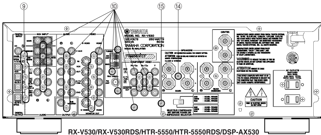
RX-V530/RX-V530RDS/HTR-5550/HTR-5550RDS/DSP-AX530
