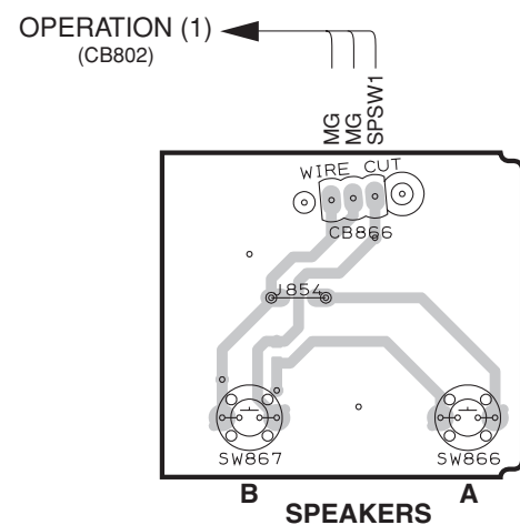
OPERATION (5) P.C.B. (Side A)
