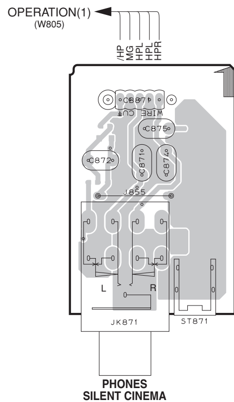
OPERATION (3) P.C.B. (Side A)
