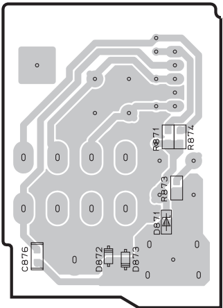
OPERATION (3) P.C.B. (Side B)
