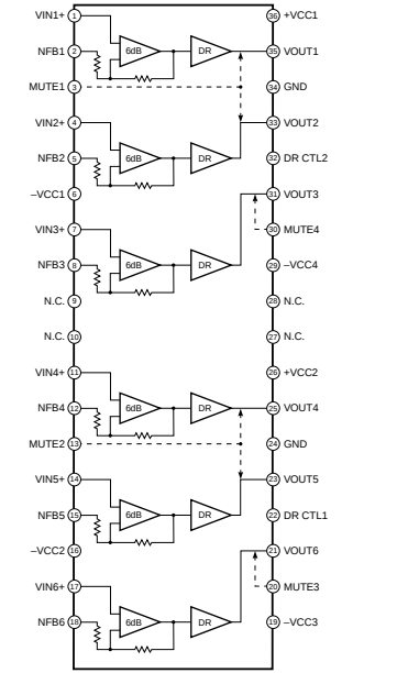
IC588 : LA7109 75Ω Video Driver
