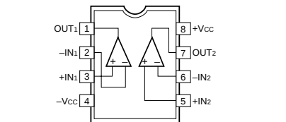
IC311, 313-317, 319, 320 : μPC4570G2 Dual OP-Amp
