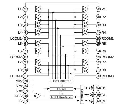
IC301, 303 : LC78211 Analog Function Switch
