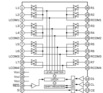
IC302, 304 : LC78213 Analog Function Switch
