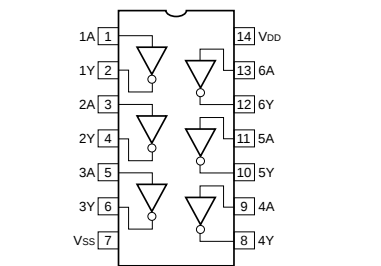
IC585 : TC74HCU04AP Hex Inverters
