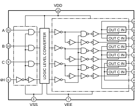
IC584, 712 : TC74HC4053AP Triple 2-Channel Multiplexer/Demultiplexer
