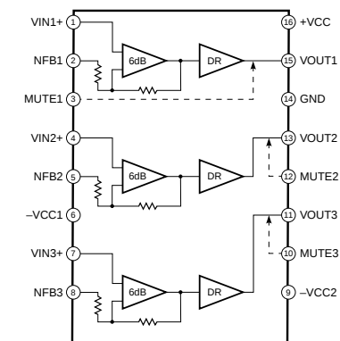
IC681 : LA7108M-TLM 75Ω Video Driver
