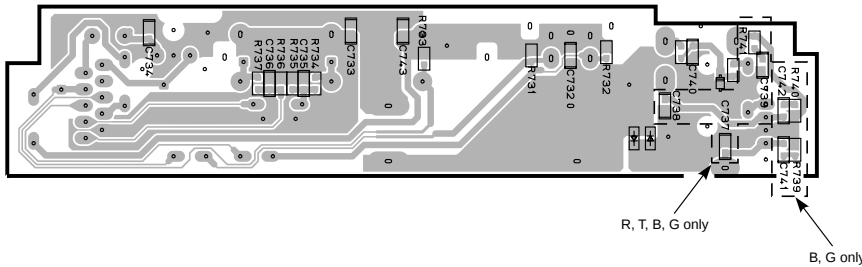
OPERATION ( 6 ) P. C. B.
