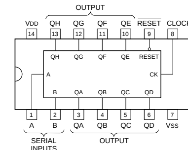
IC586 : TC74HC164AF-EL 8-Bit Shift Register
