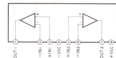
IC507 , 508 : \mu PC4570HA Dual OP-Amp
