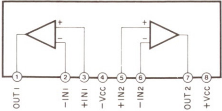
IC507 , 508 : \mu PC4570HA Dual OP-Amp
