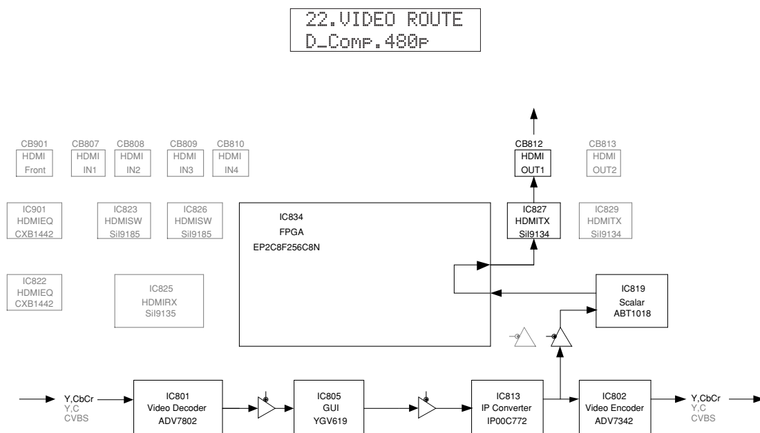
Component_480p to DA and HDMI_out1
