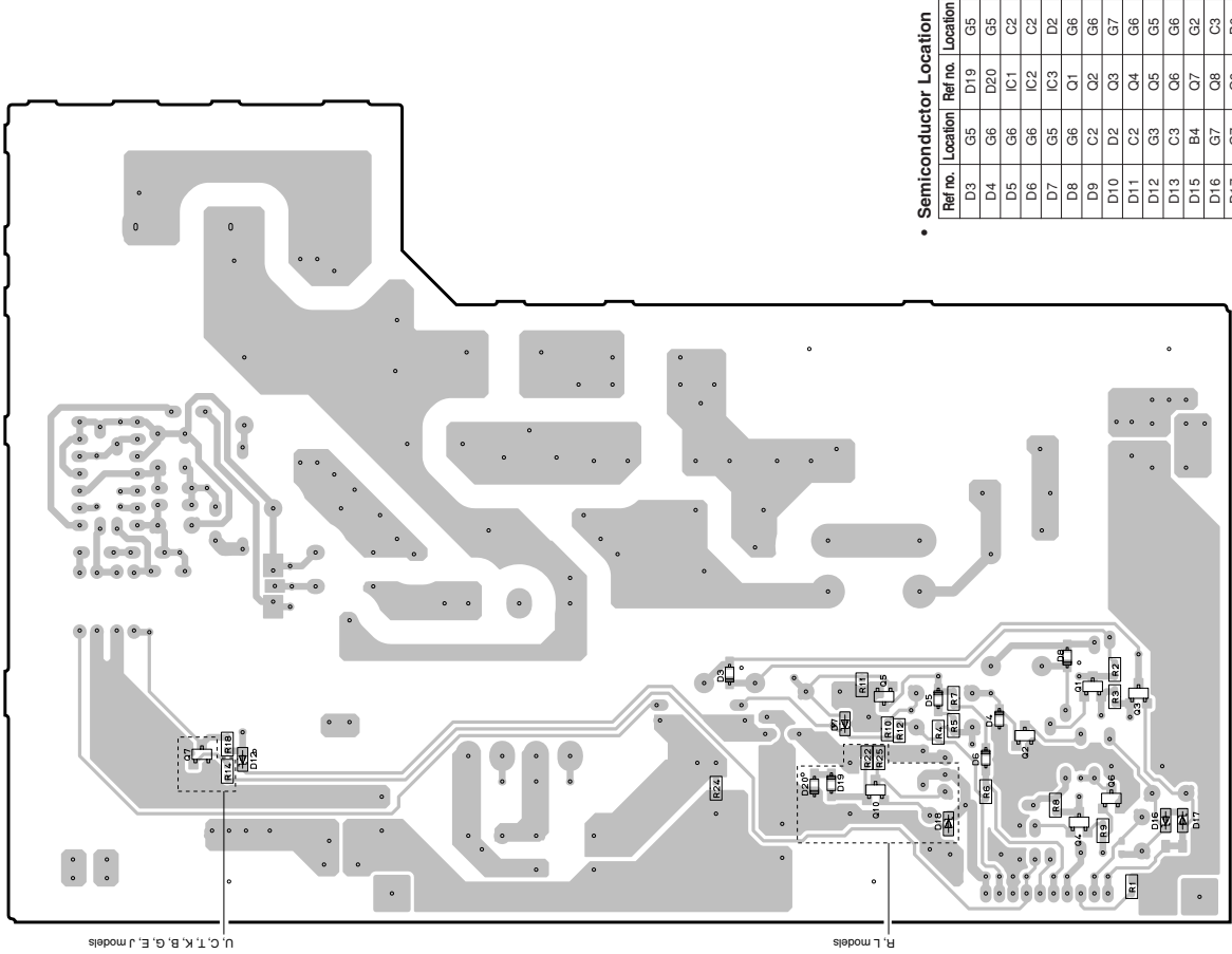
POWER (1) P.C.B. (Side B)
