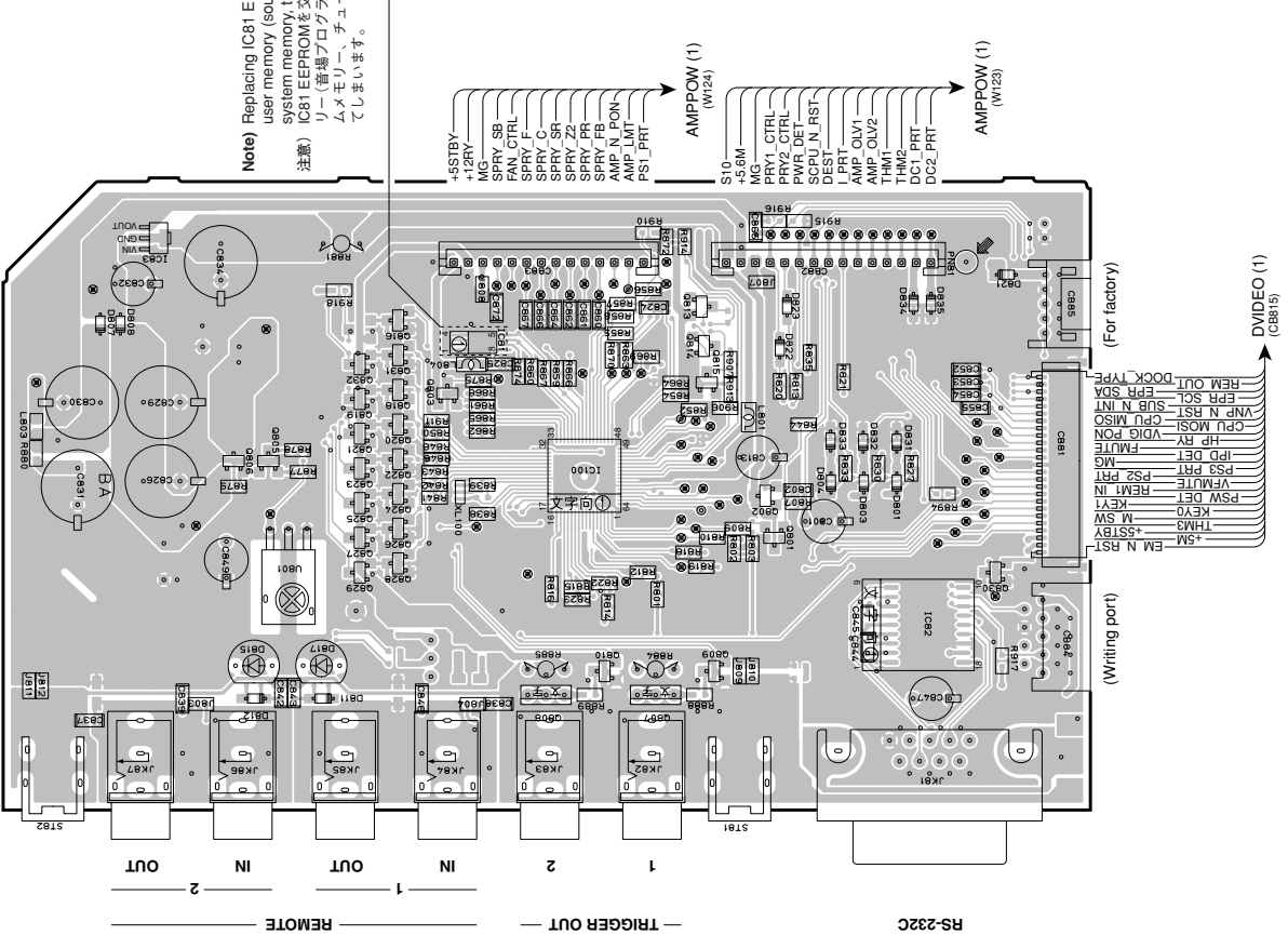
SUBCPU (1) P.C.B. (Side A)
