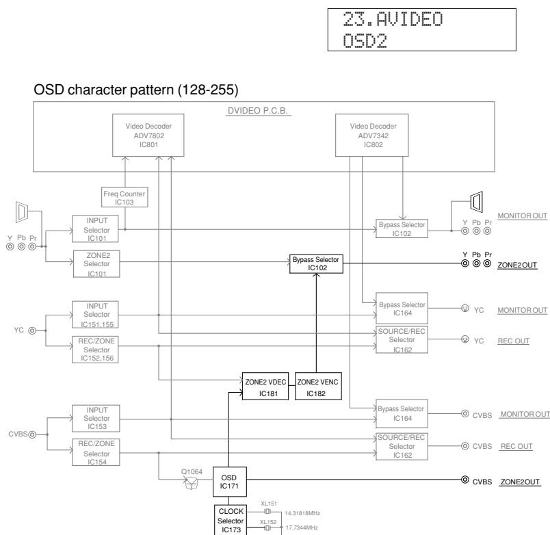
OSD character pattern (128-255)
