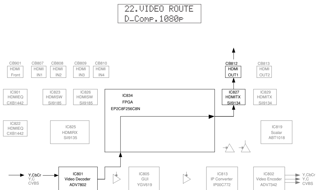
Component_1080p to HDMI_out1
