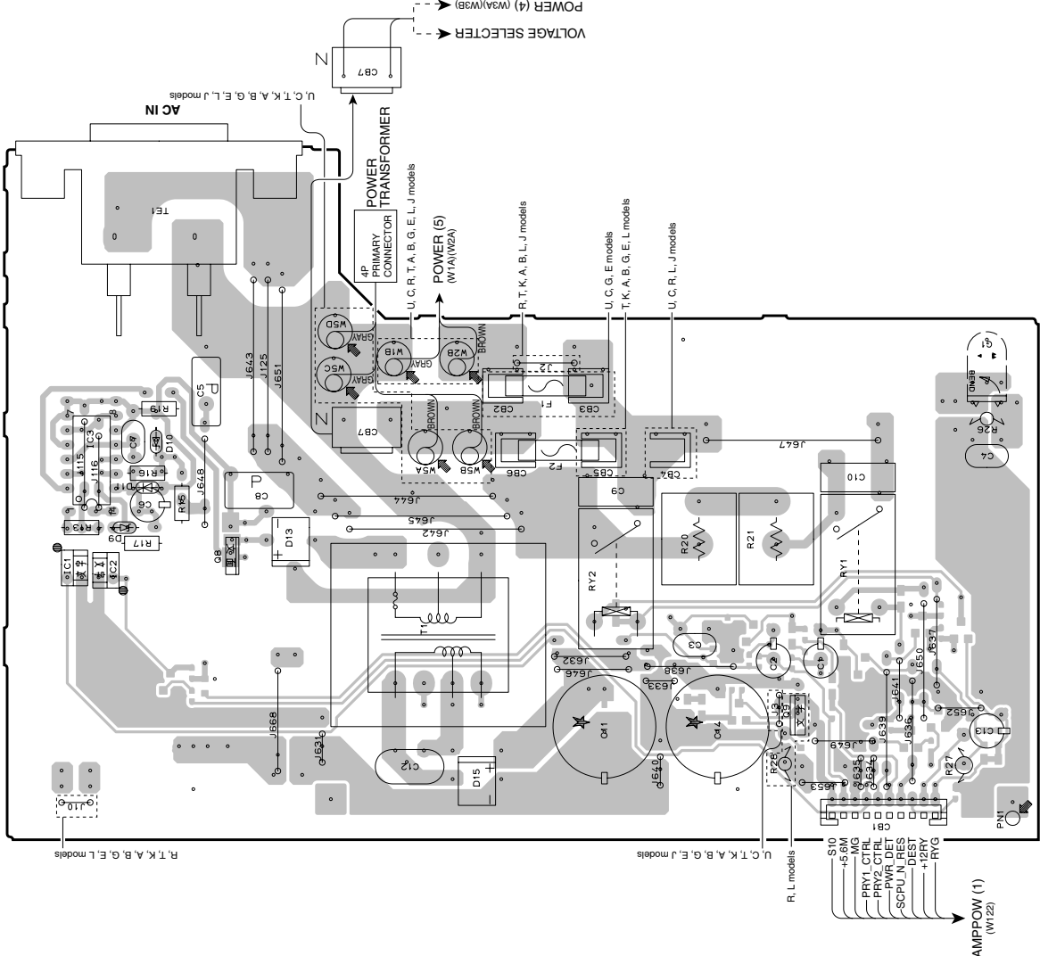
POWER (1) P.C.B. (Side A)
