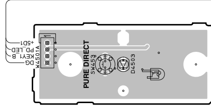
OPERATION (3) P.C.B.
