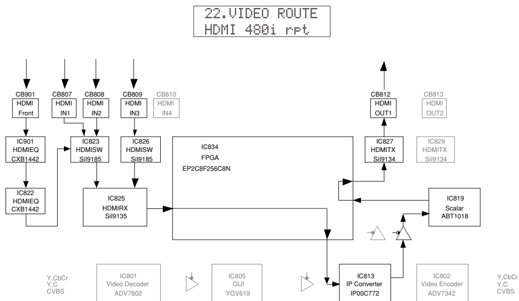
HDMI_480i to HDMI_out1
