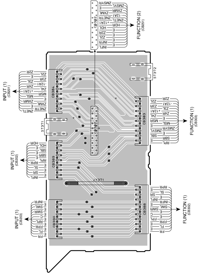
SUBCPU (3) P.C.B. (Side A)
