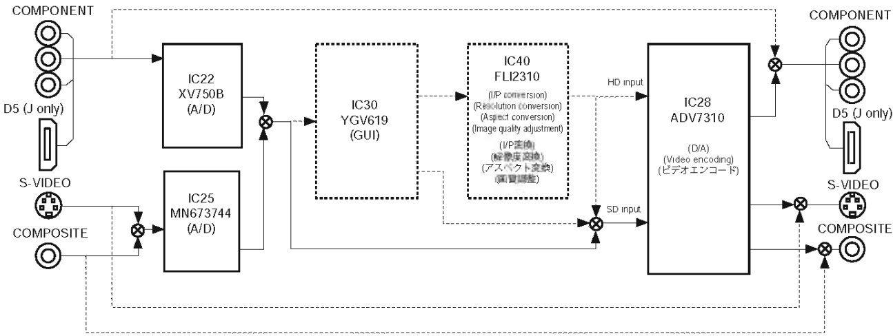
9.VIDEO DIGITAL BYPASS
