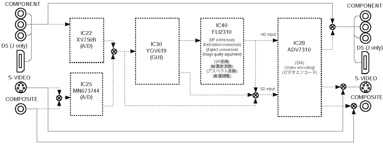
9.VIDEO ANALOG BYPASS
