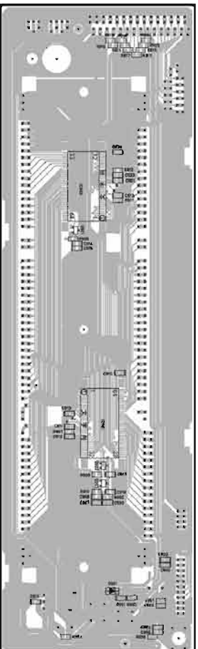
OPERATION (1) P.C.B.
