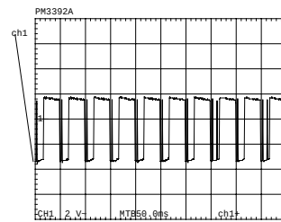
TP 17: SCL
