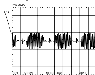
TP 21: C_OUT
