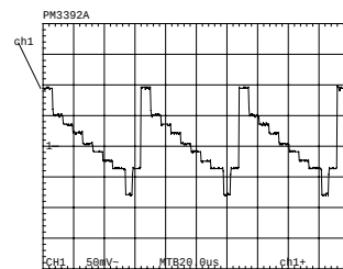
TP 20: Y_OUT
