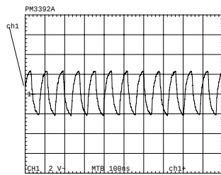
TP 10: PCM_CLK
