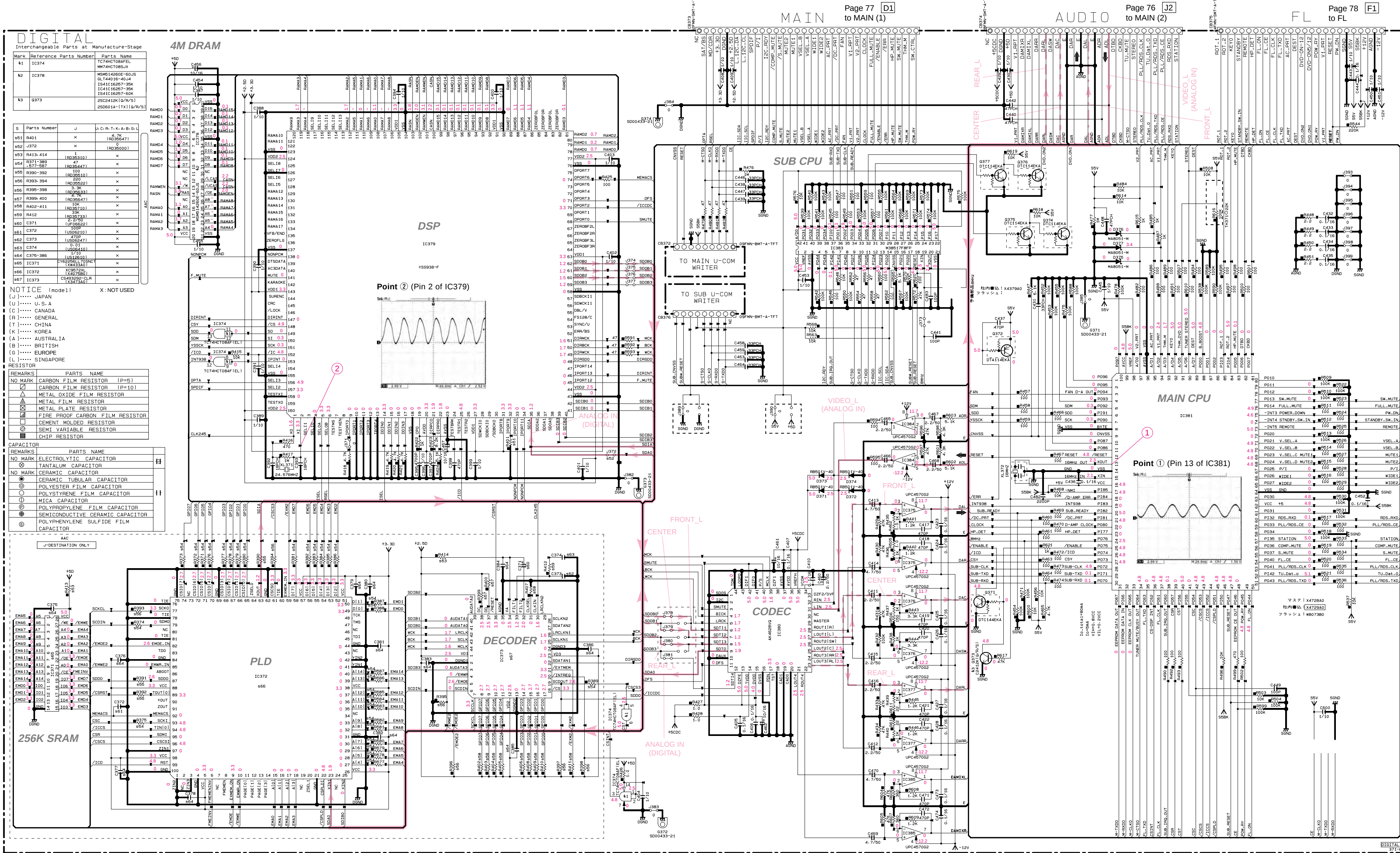
IC371 : CV62256LL-70SNCT Static RAM
