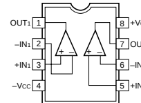
IC311 : NJM2904M IC701 : \mu PC4570G2 Dual OP-Amp
