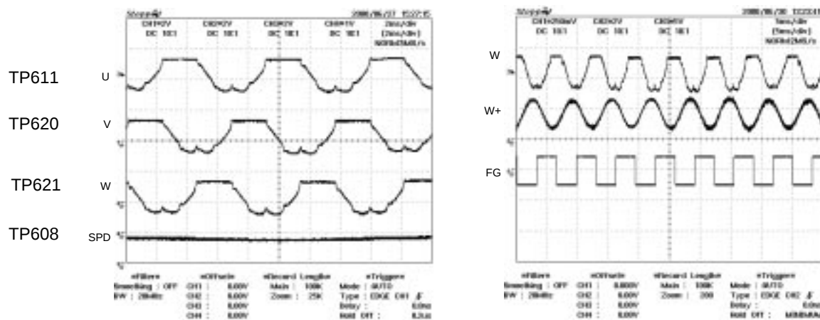
Spindle (W, W+, FG)
