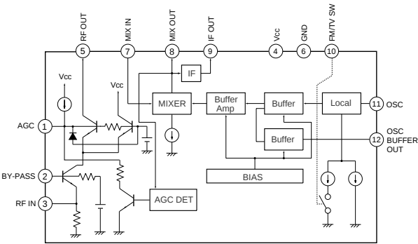
IC201 TA8176SN (FM Front End)
