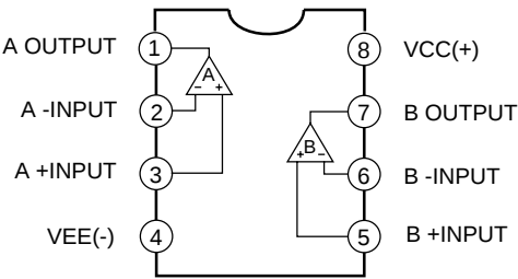
IC211~213 NJM4558M (Operational Amplifier)
