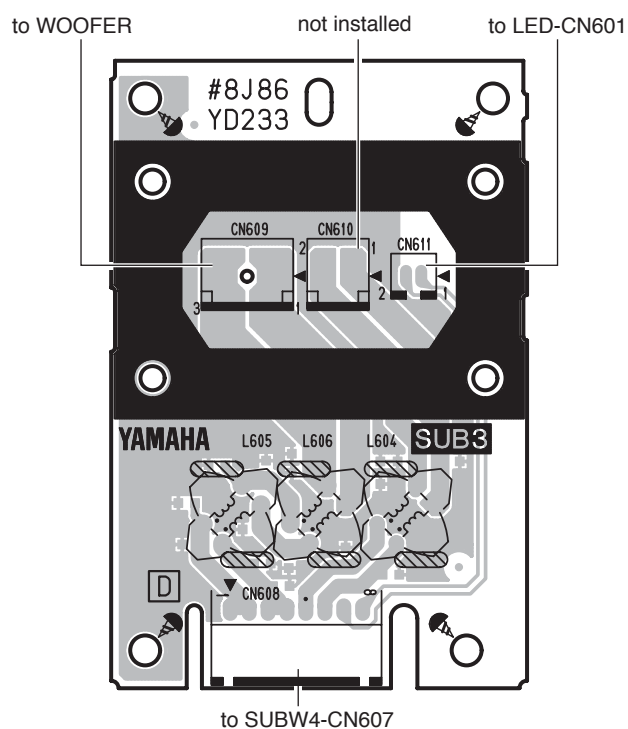
Component side (部品側)
