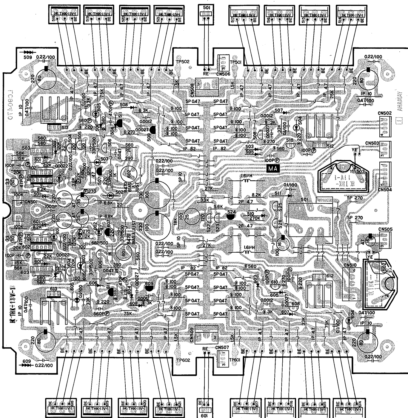
Tr 501, 601 2SA979 (G) Tr 514 ~ 517, 614 ~ 617 2SC2581 (O, Y) Tr 502, 602 2SA995 (G) Tr 518 ~ 521, 618 ~ 621 2SA1106 (O, Y) Tr 503, 603 2SC2291 (G) Tr 526 2SD667 (B, C) Tr 504, 506, 522, 523, 525, 604, 606 2SC1815 (GR) D501 ~ 504, 601 ~ 604 1S2473 Tr 505, 510, 605, 610 2SC2704 (O, Y) D505 ~ 508, 605 ~ 608 1SS82 Tr 507, 511, 607, 611 2SA1144 (O, Y) D509, 609 STV-3H Tr 508, 608 2SC2240 (GR, BL) D510, 511 10D1 Tr 509, 524, 609 2SA970 (GR, BL) ZD501, 601 RD24EB2 Tr 512, 612 2SC2238 (O, Y) LED501 ~ 505, 601 ~ 605 LTZ-R17 Tr 513, 613 2SA968 (O, Y) RY501 MSJ12D2-0 TH501, 601 STR60R70
