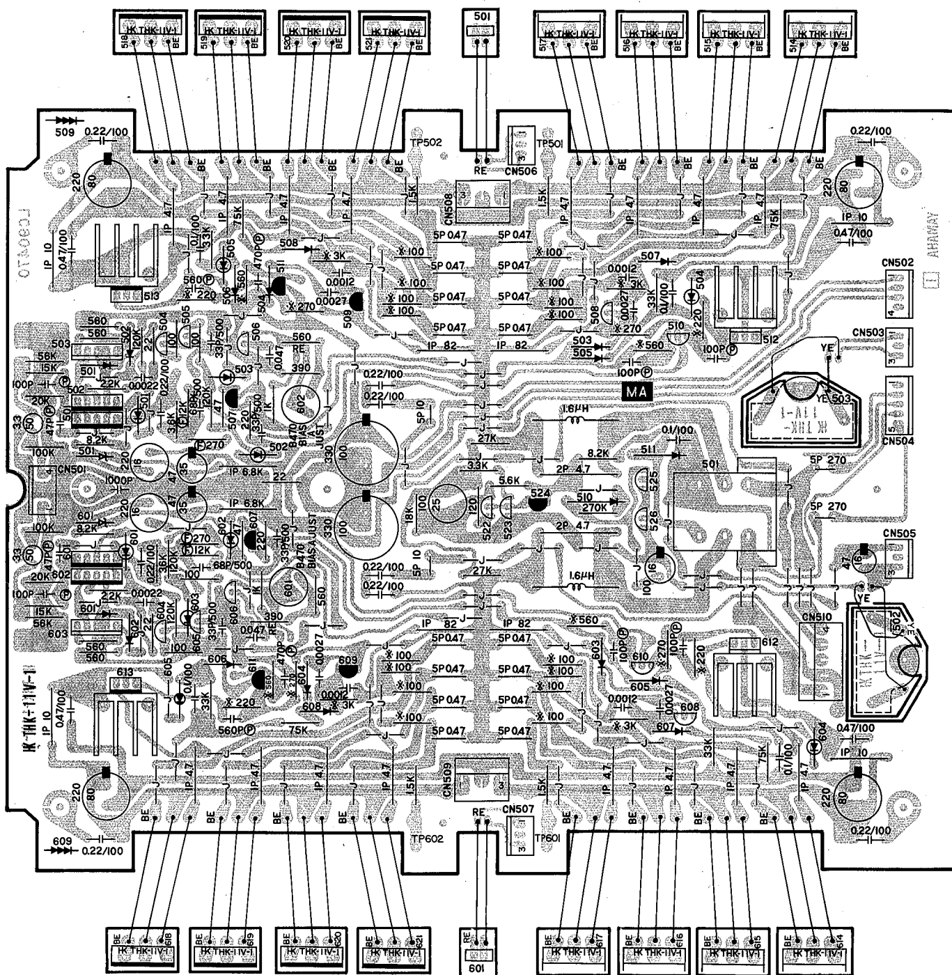
MA2 CIRCUIT BOARD
