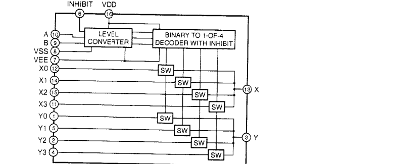
IC213 : TC4052BP Dual 4 Channel Analog Multiplexers/Demultiplexers
