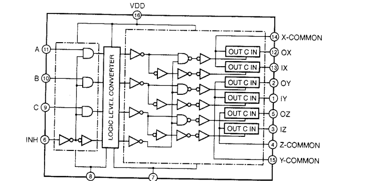
IC216 : TC4053BP Triple 2 Channel Analog Multiplexers/Demultiplexers
