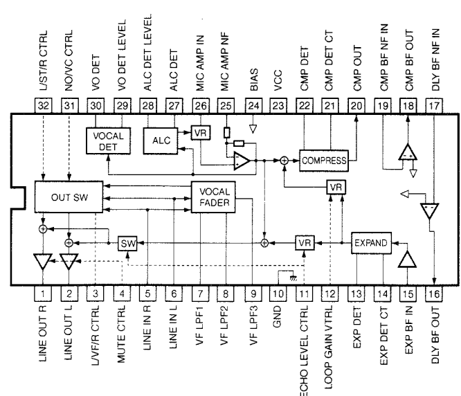
IC210 : BA7726AS Analog Componder for Karaoke Echo System
