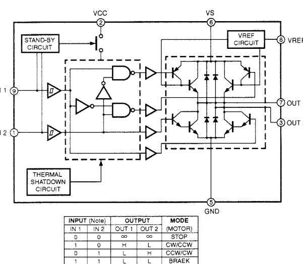
IC203, 204 : TA8409S Full Bridge Motor Driver
