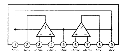
IC207 : \mu PC4570HA Dual OP-Amp
