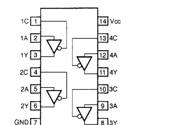
IC208 : HD74HC125P Quad 3 State Bus Buffers
