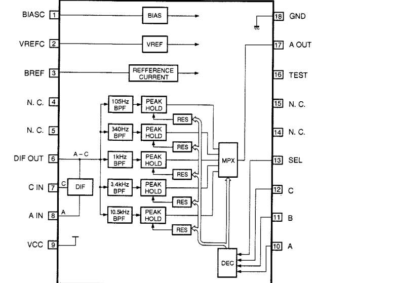
IC215 : BA3835S 5-Band BPF and Peak Hold for Spectrum Analyzer
