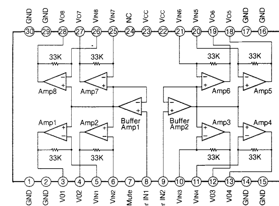
IC202 : LA6536M 4 Channel BTL Driver
