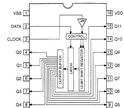
IC218 : BU2090 Serial In/Parallel Out Driver
