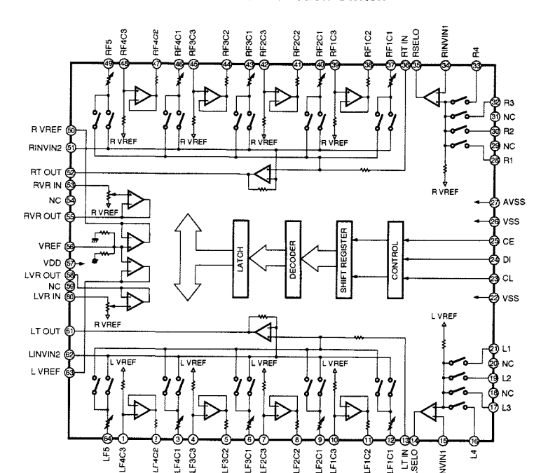
IC215 : BA3835S 5-Band BPF and Peak Hold for Spectrum Analyzer
