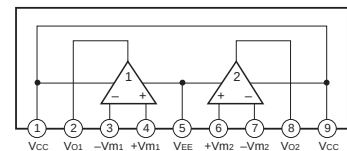
IC802, 806, 810 : \mu PC4570HA Dual OP-Amp
