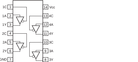
IC7, 9 : TC74HC125AF Quad 3 State Bus Buffers
