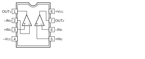
IC10 : μPC4570G2 Dual OP-Amp
