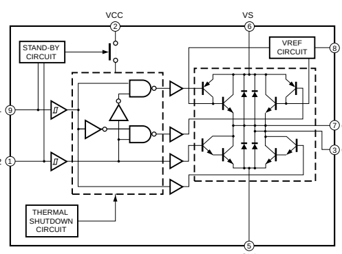
IC3, 4 : TA8409S Full Bridge Motor Driver
