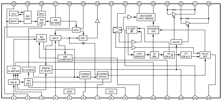
IC1 : LA1838 AM/FM Tuner
