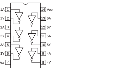
IC13 : TC74HC04AF Hex Inverters
