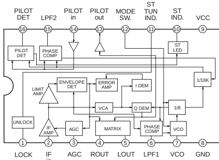
IC3 : TA2040AF AM Stereo Demodulator
