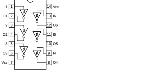
IC8 : TC74VHC14F Hex Schmitt Trigger Inverters
