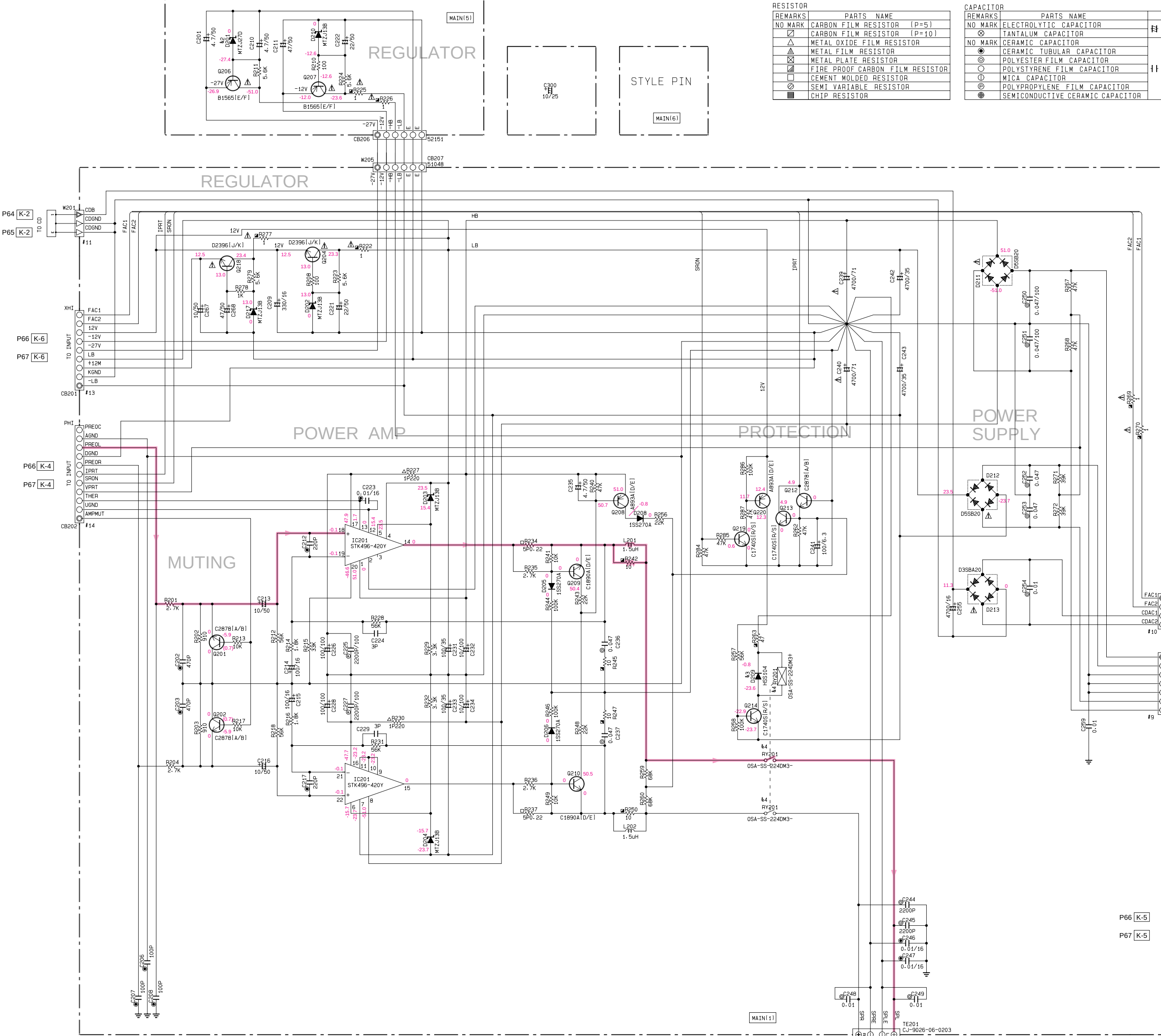
IC201 : STK496-420Y 2 Channel AF Power Amp
