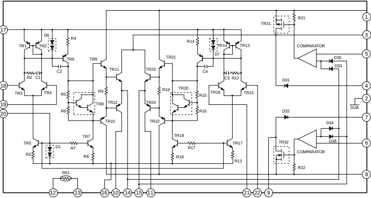
IC201 : STK496-420Y 2 Channel AF Power Amp
