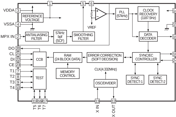
IC4 : LC72720NM RDS Decoder & Controller
