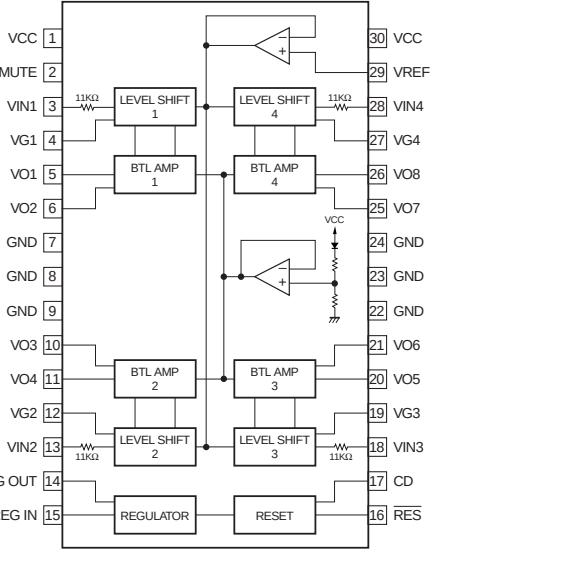
IC1 : LA6541D 4 Channel BTL Driver
