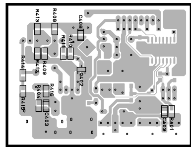
GX-505VCD INPUT P.C.B. (2) (Surface Mount Device)
