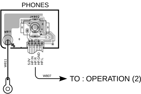
OPERATION P.C.B. ( 4 )
