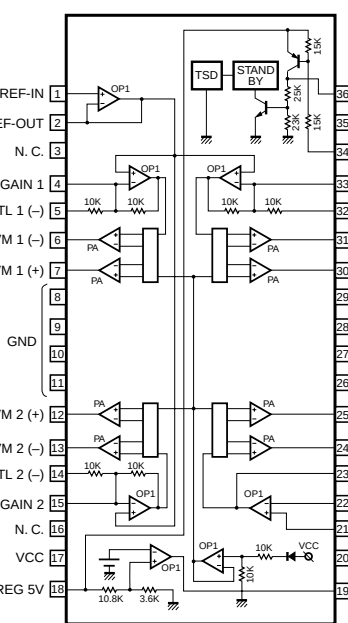
IC1 : M56748FP 4 Channel BTL Driver
