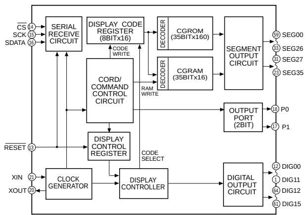
IC803 : M6604MASP FL Driver
