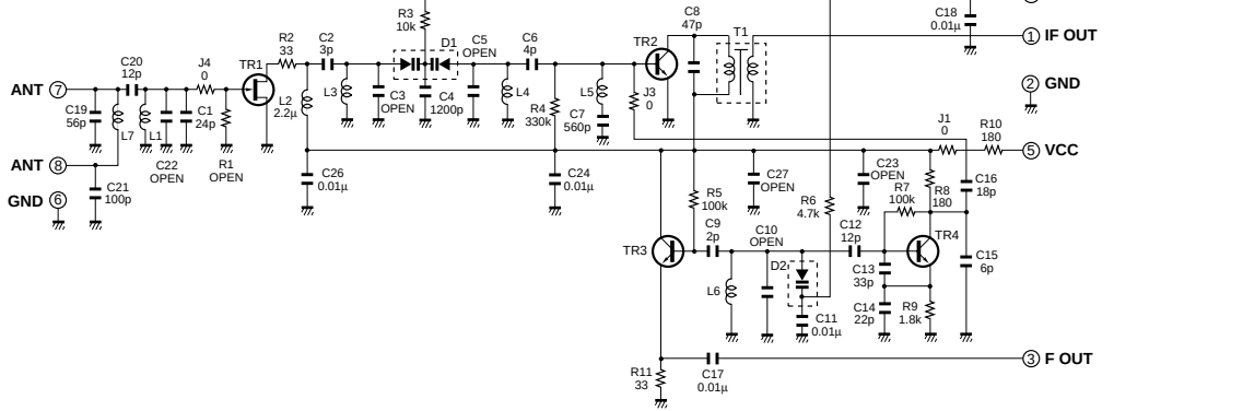
PK1 : TFFJ4E515A (VU134500) A, B, G models
