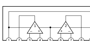
IC805-807 : μPC4570HA Dual OP-Amp
