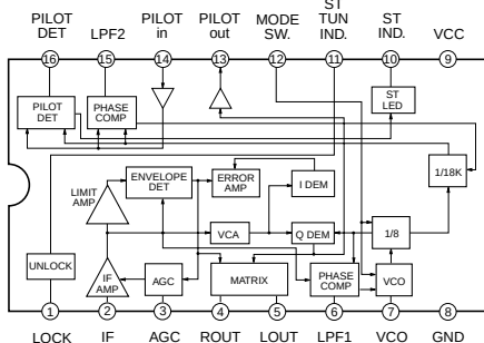
IC3 : TA2040AF AM Stereo Demodulator
