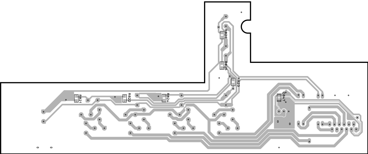
OPERATION P.C.B. ( 5 )
