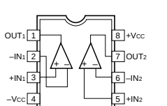
IC13, 14 : μPC4570G2 Dual OP-Amp
