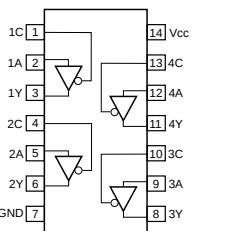
IC9 : TC74HC125AF Quad 3 State Bus Buffers
