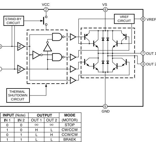
IC2, 3 : TA8409S Full Bridge Motor Driver
