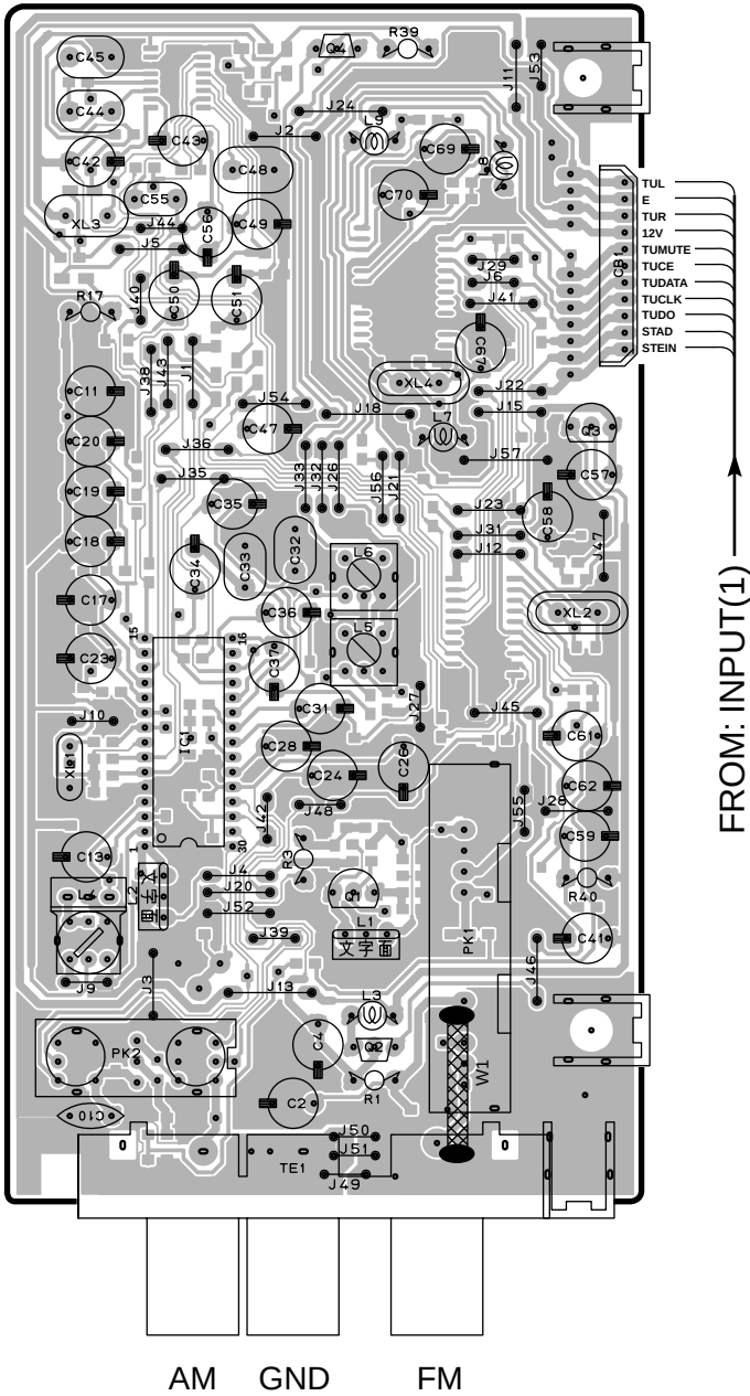
TUNER P.C.B. (Lead Type Device)
