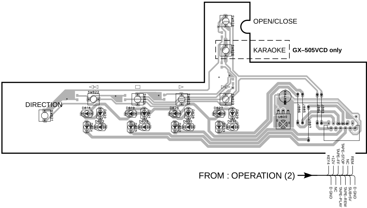
OPERATION P.C.B. ( 5 )
