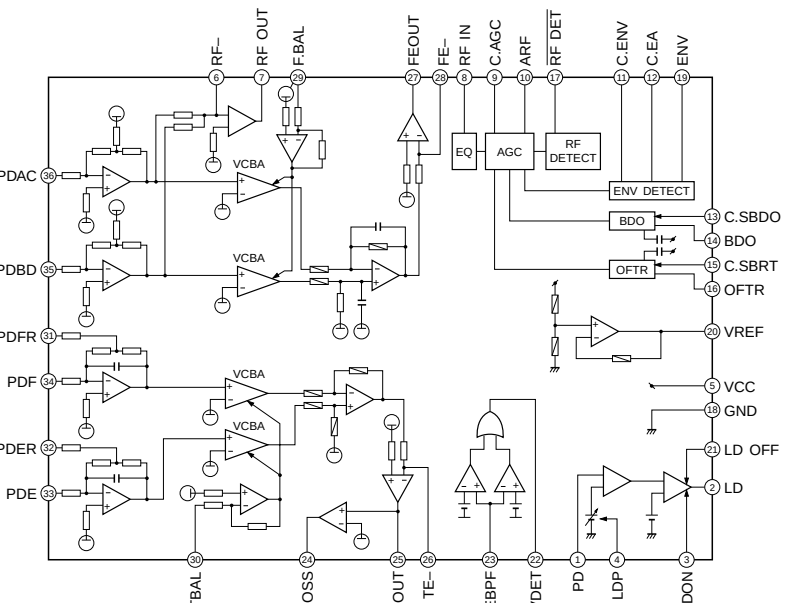
IC4 : AN8806SB Digital Servo Head Amp
