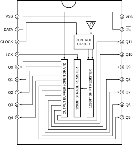
IC802 : BU2092 Serial In/Parallel Out Driver
