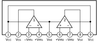
IC807 : μPC4570HA Dual OP-Amp
