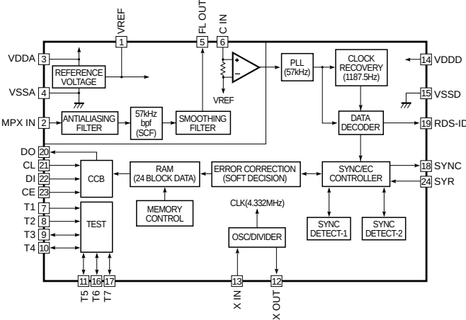
IC4 : LC72720NM RDS Decoder & Controller
