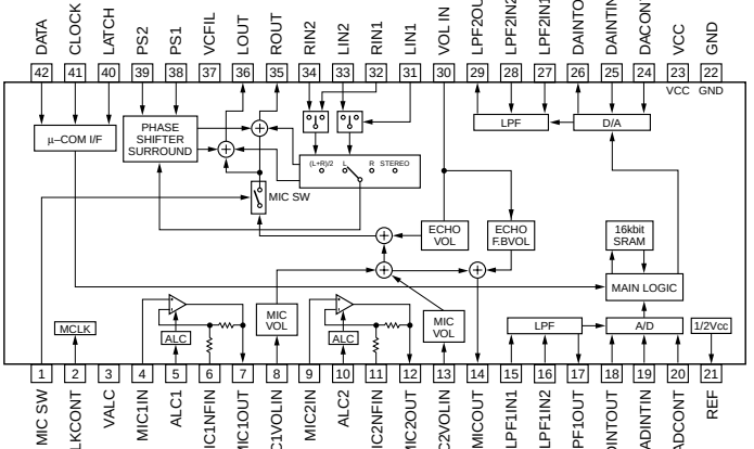
IC800 : M65853FP Mic Amp with Digital Echo
