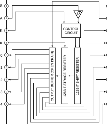
IC802 : BU2092 Serial In/Parallel Out Driver
