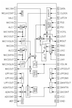
IC801 : MS8887P MIC Amp with Digital Echo
