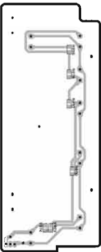
P.C.B. OPERATION(4) (Surface Mount Device)
