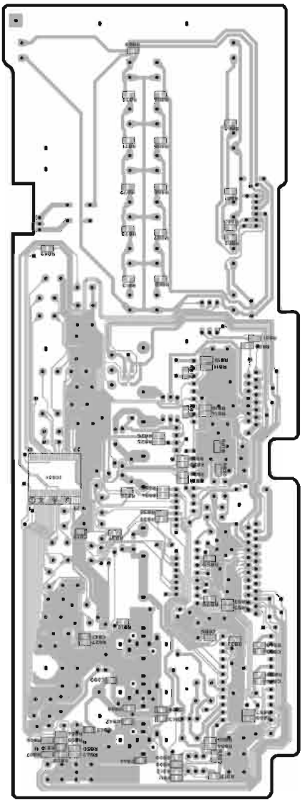
GX-700VCD P.C.B. OPERATION(3) (Surface Mount Device)
