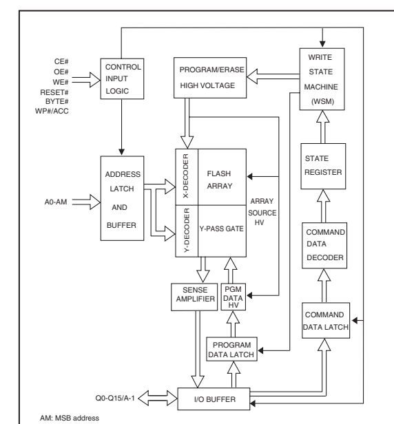
IC243: MX29LV160BTI-70G 16M-bit 3V supply flash memory
