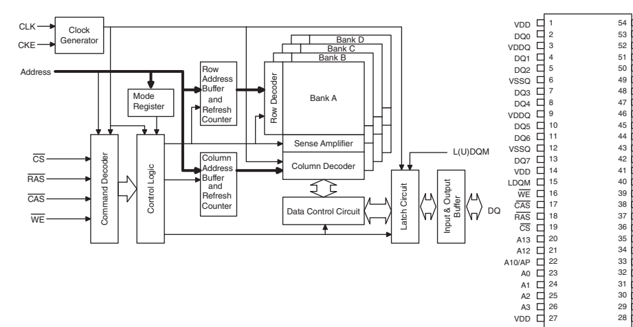
IC242: M12L64164A-5TG 1M x 16-bit x 4 banks synchronous DRAM
