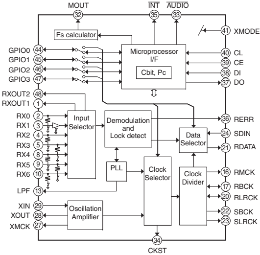
IC261: LC89058WD-E Digital audio interface receiver
