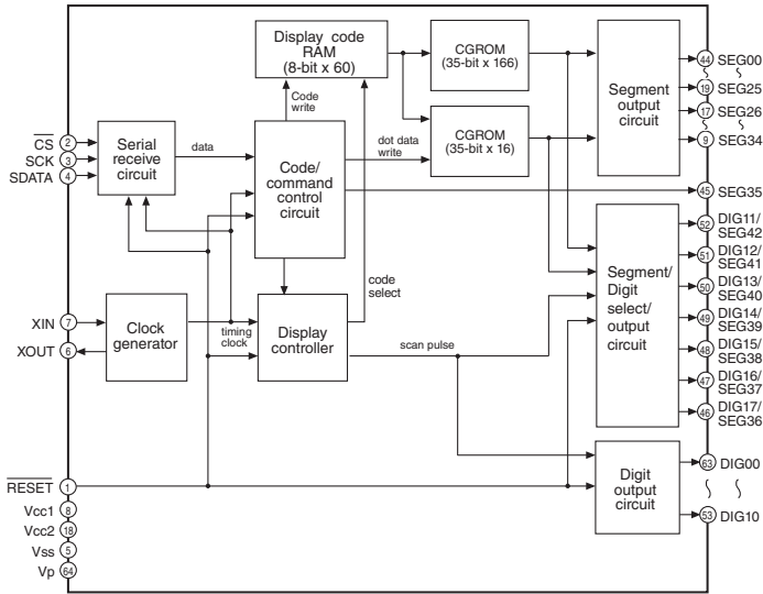
IC101: M66003-0131FP-R 18 digit 5 x 7 segment VFD controller/driver
