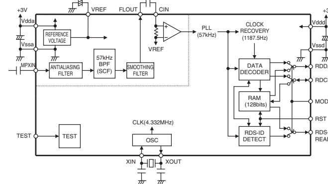
IC223: LC72725KM-UY-TLM-E RDS signal demodulation IC
