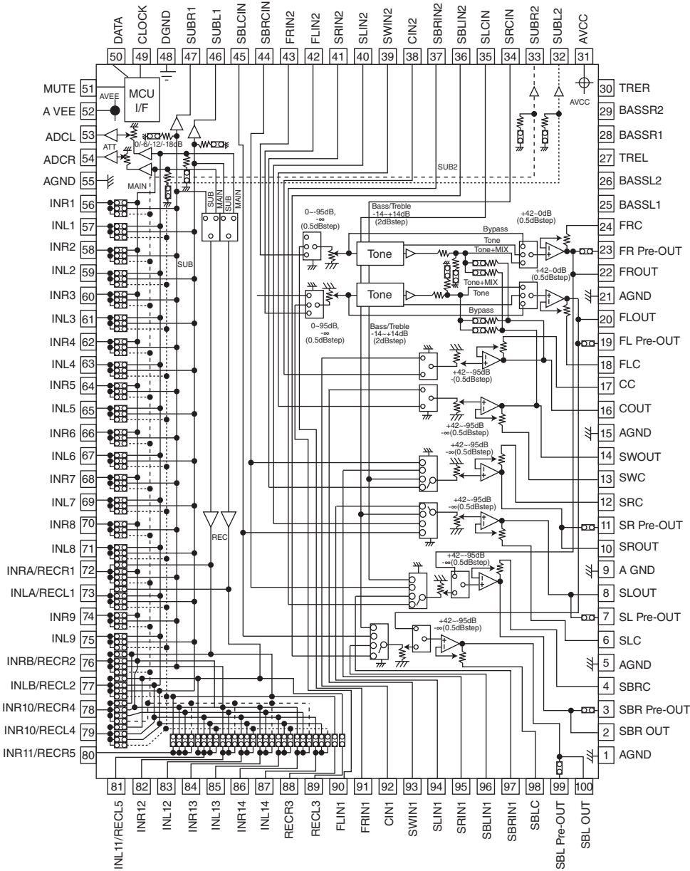
IC21: R2A15220FP 8-channel electronic volume with 11 input selector and tone control
