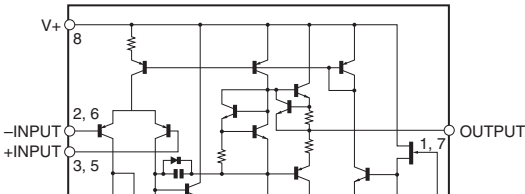
IC102: NJM4565M (TE1) Dual operational amplifier
