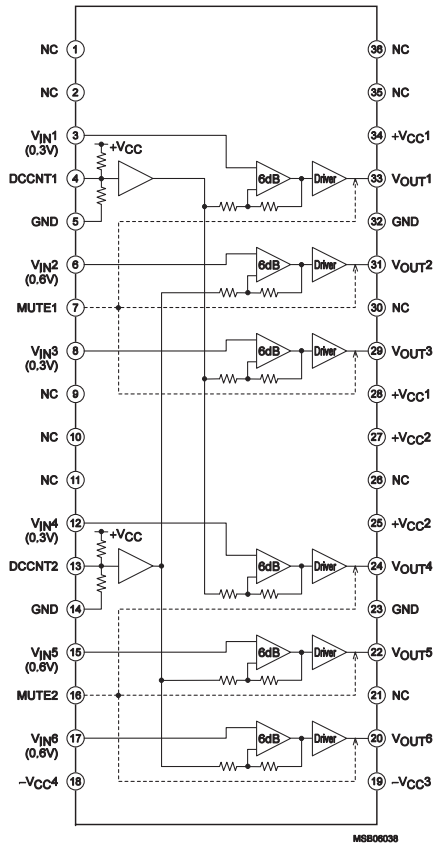
IC43: LA73050-TLM-E 6-channel 75-ohm video driver
