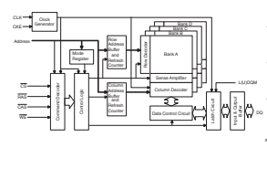
IC242: M12L64164A-STG 1M x 16-bit x 4 banks synchronous DRAM
