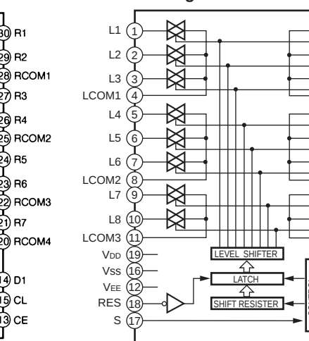
IC103 : LC78212 Analog Function Switch
