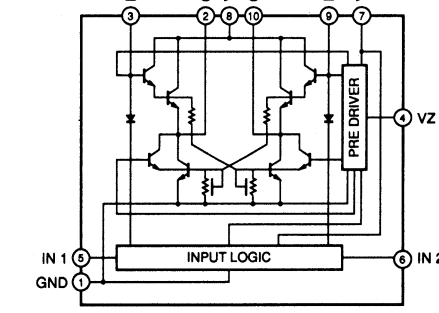
IC404 : LB1641 Motor Driver
