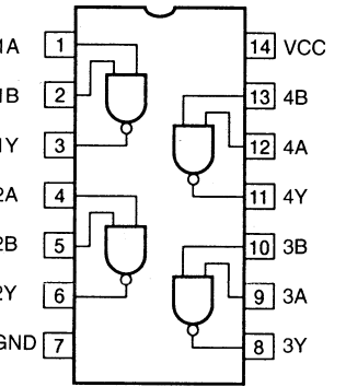
IC352 : HD74HC00P Quadruple 2-input Positive NAND Gates
