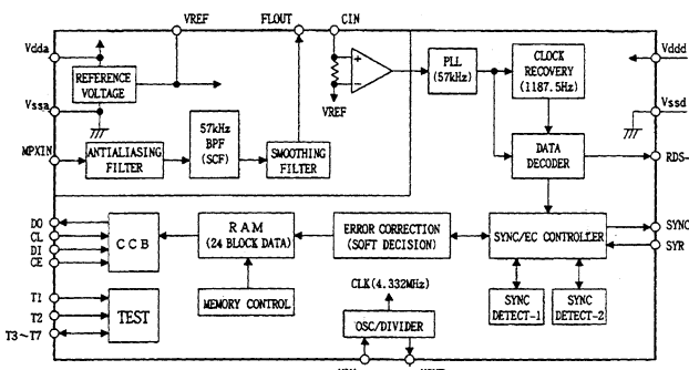
IC4 : LC72720N RDS Decoder & Controller
