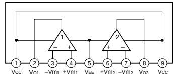
IC202 : μPC4570HA Dual OP-Amp
