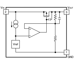
IC1 : RH5E58AA-T1-FA Voltage regulator
