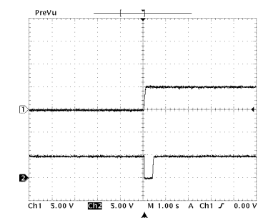
POINT (B-2) ①/ Pin7, ②/ Pin8 of CB3
