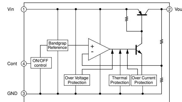
IC100, 102, 106 : NJM2388F Low dropout voltage regulator with ON/OFF control
