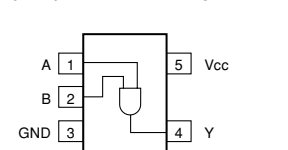
IC6 : SN74AHC1G08DCKR 2-input positive-AND gate
