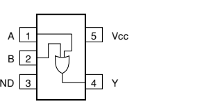
IC4, 5 : SN74AHCT1G32DCKR Single 2-input positive-OR gate
