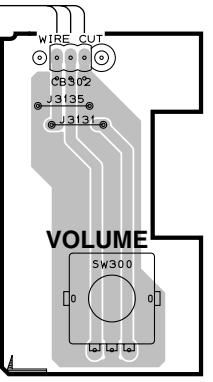
OPERATION (6) P.C.B. (Side A)
