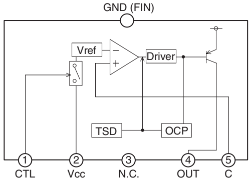
IC601: BA00BC0WFP-E2 1.0 A low-dropout voltage regulator with shut down switch
