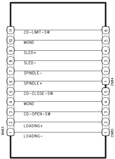
FRONT/SMPS (2)
