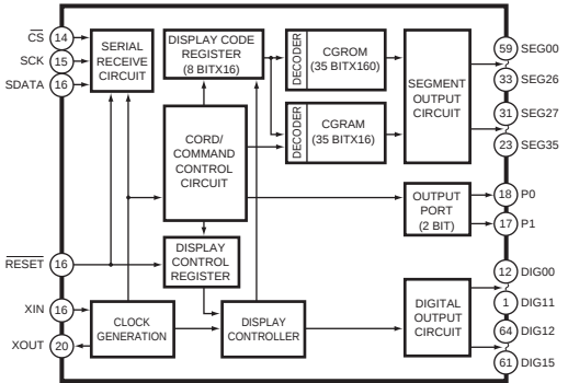
SUB IC801
