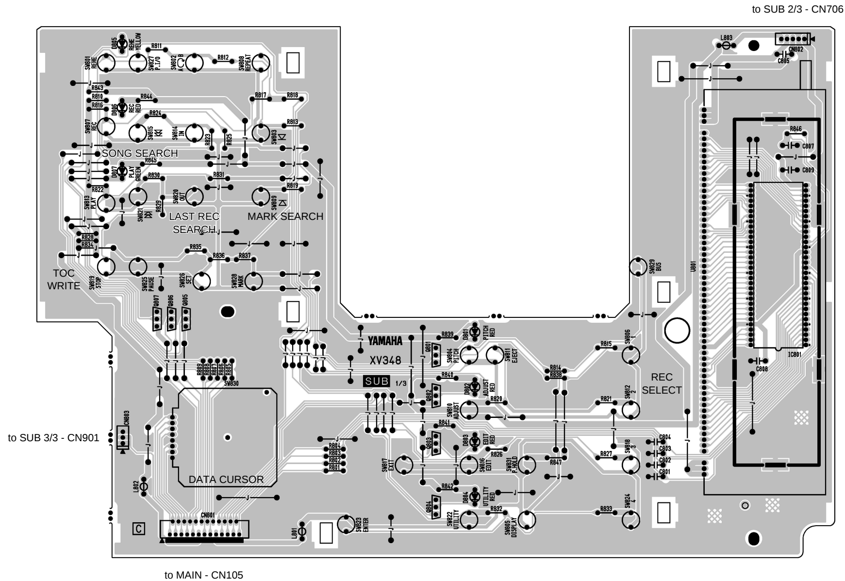
Component side
