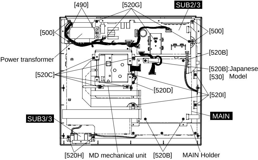
[490]: Bind Head Screw 4.0 X 8 MFZN2BL (EG340360) [500]: Bind Head Tapping Screw-P 4.0 X 12 MFZN2BL (VA847600) [520]: Bind Head Tapping Screw-B 3.0 X 8 MFZN2BL (EP600190) [530]: Screw 3B-8Y9294 (VR602100)
