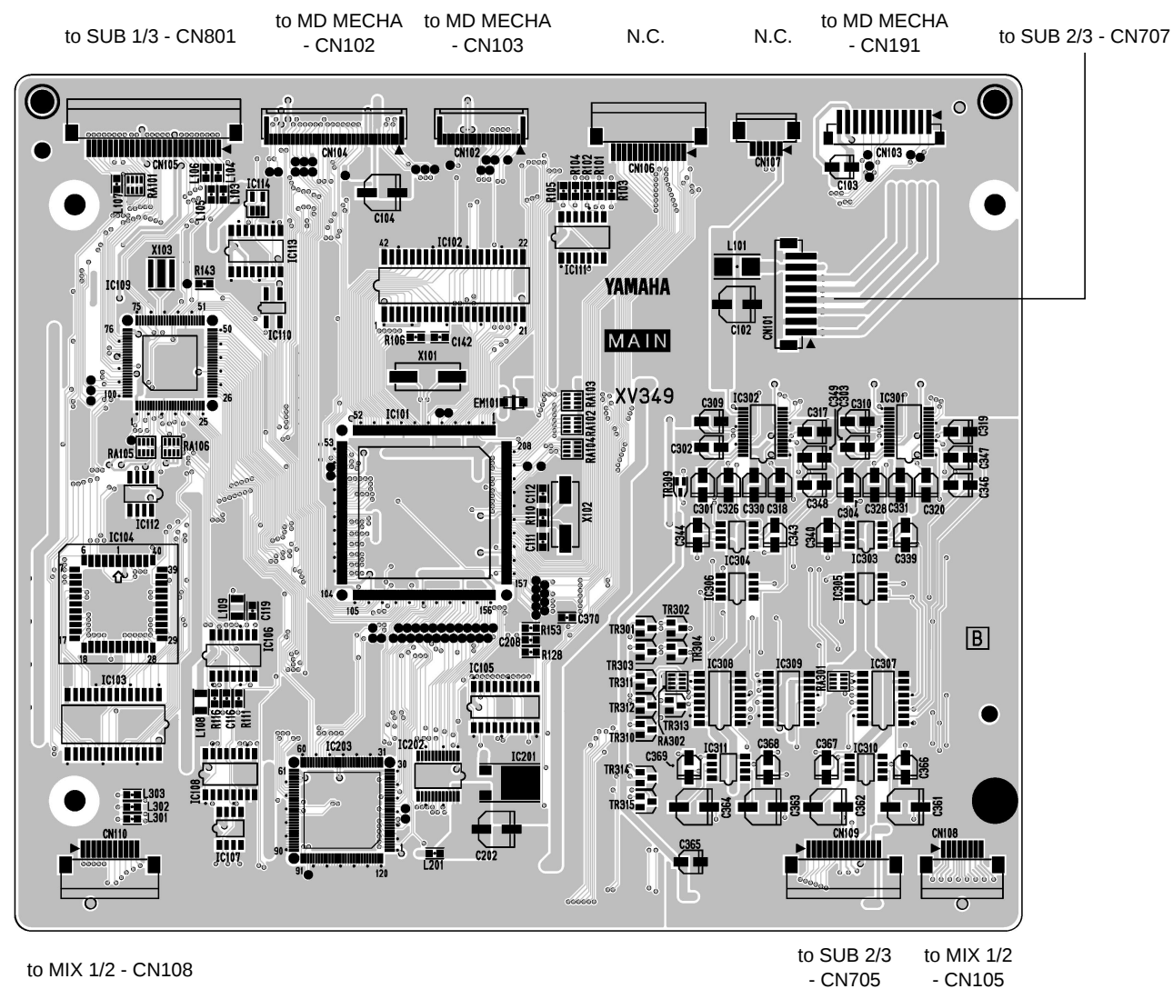
Component side
