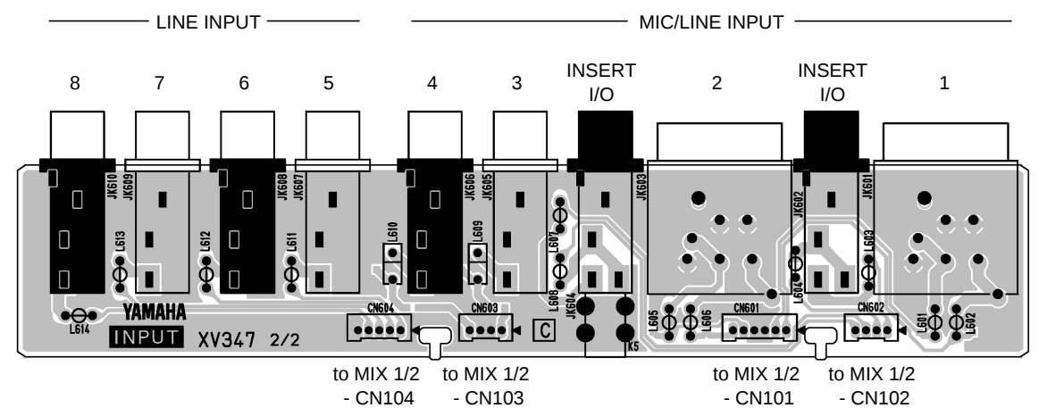
Component side
