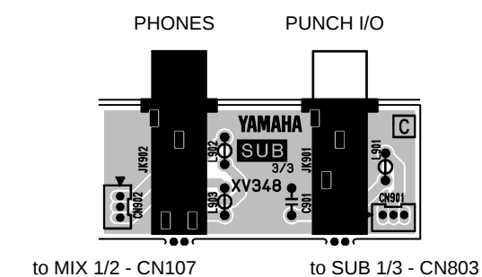
Component side
