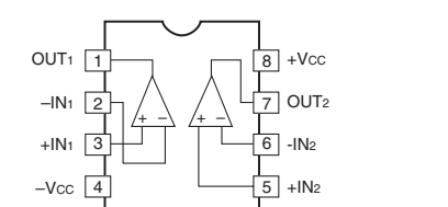
IC304, 305, 307, 310: NJM2068MD-TE2 Dual operational amplifier
