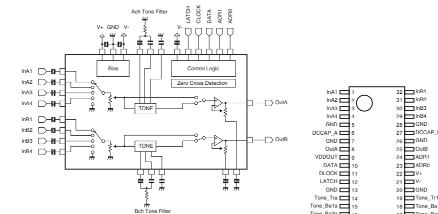
IC303: NJW1194V 2-channel electronic volume input selector and tone control
