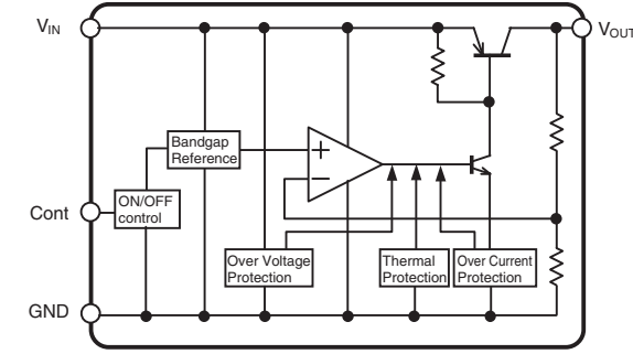
IC1: NJM2388F05 Low dropout voltage regulator with ON/OFF control
