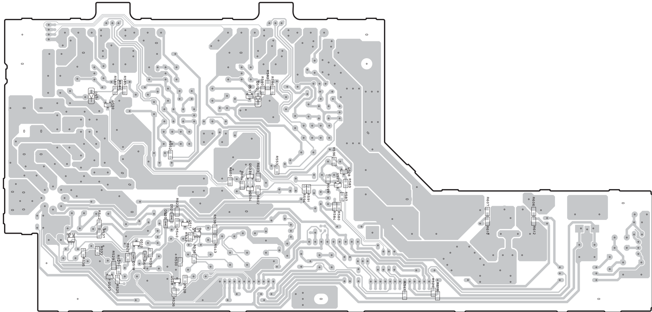
MAIN (1) P.C.B. (Side B)
