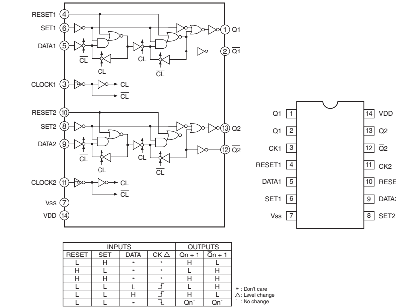
IC4: TC4013BP Dual D-type flip flop
