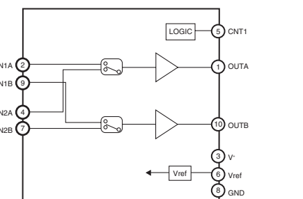
IC302: NJM2752RB0 2-input/1-output stereo audio selector
