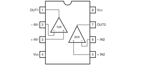
IC308: BA15218F Dual high slew rate, low noise operational amplifier
