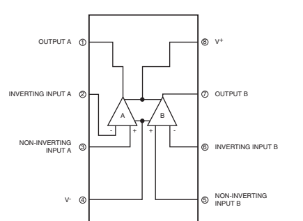
IC306: LME49723MAX/NOPB Dual high fidelity audio operational amplifie
