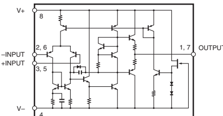
IC309: NJM4580E Dual operational amplifier
