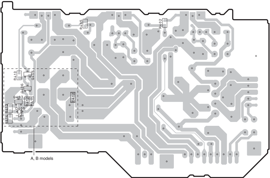
MAIN (2) P.C.B. (Side B)
