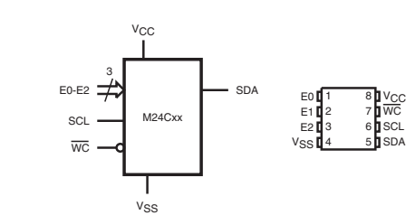
IC102: M24C02-RDW6TP 2 K-bit and 1 K-bit serial I2C bus EEPROM
