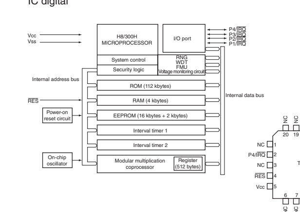
IC103: MF1341S2164 IC digital
