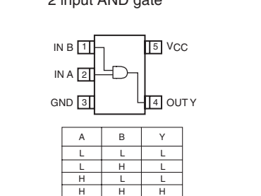
IC105, 106: TC7SET08FU 2 input AND gate
