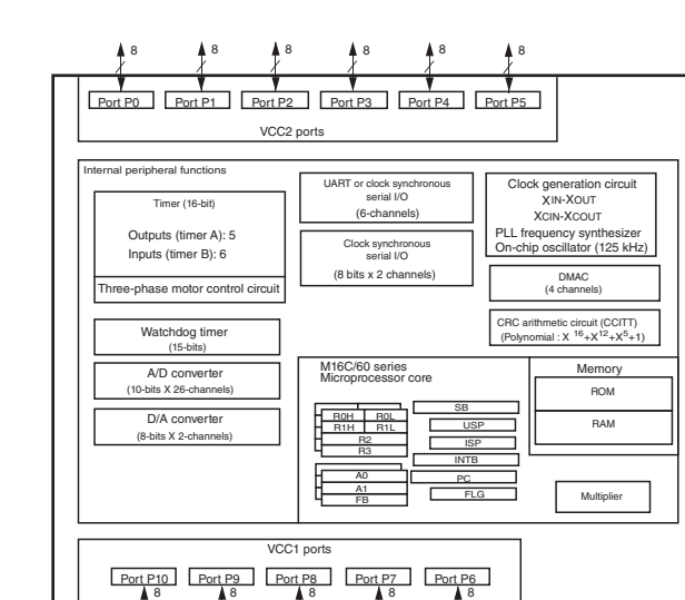
IC101: RSF3640DNFA Single-chip 16-bit CMOS microprocessor
