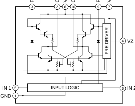
IC103 : LB1641 Motor Driver
