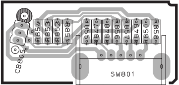
OPERATION (6) P. C. B.
