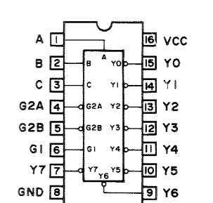
IC351 : \mu PD74HC138C 3-to-8-Line Demultiplexer
