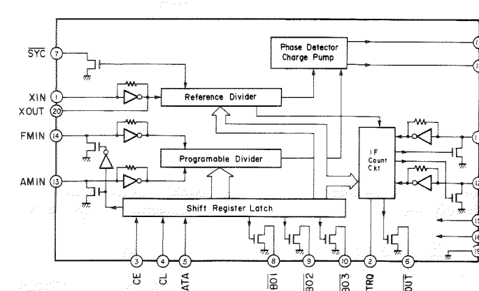
IC2 : LM7000N PLL Controller
