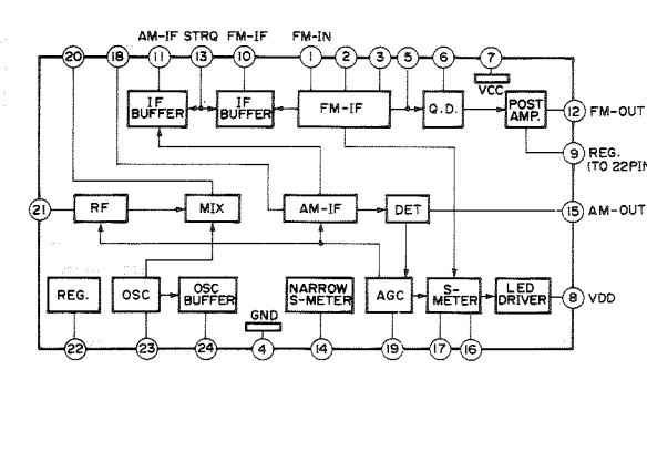
IC1 : LA1266 AM/FM IF
