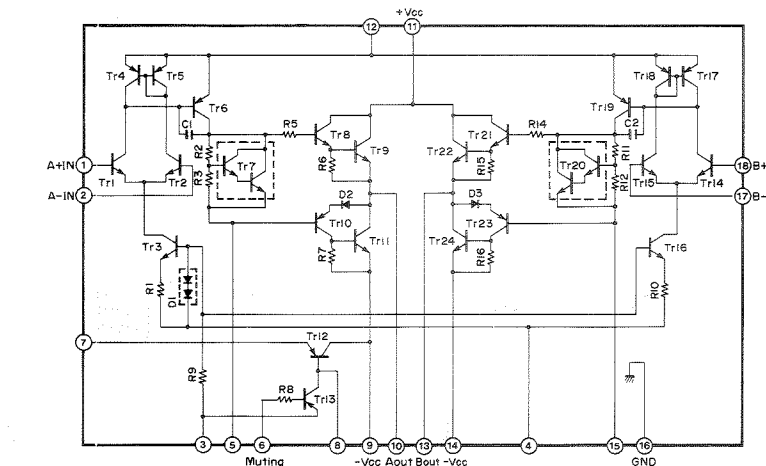
IC104 : STK4151 Power Amp
