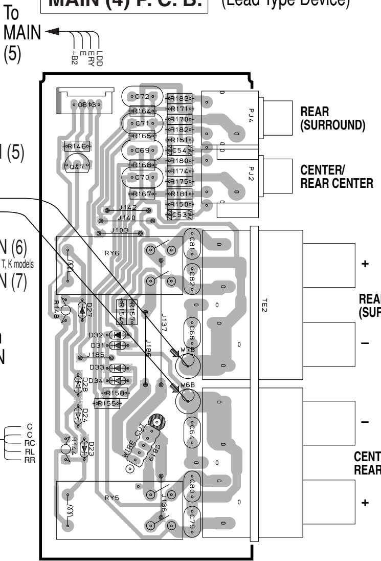
MAIN (4) P. C. B. (Lead Type Device)
