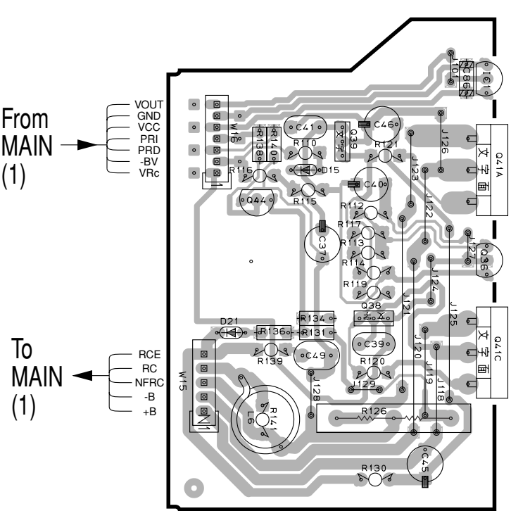
MAIN (2) P. C. B. (Lead Type Device)
