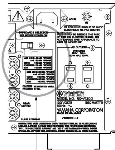
IMPEDANCE SELECTOR
