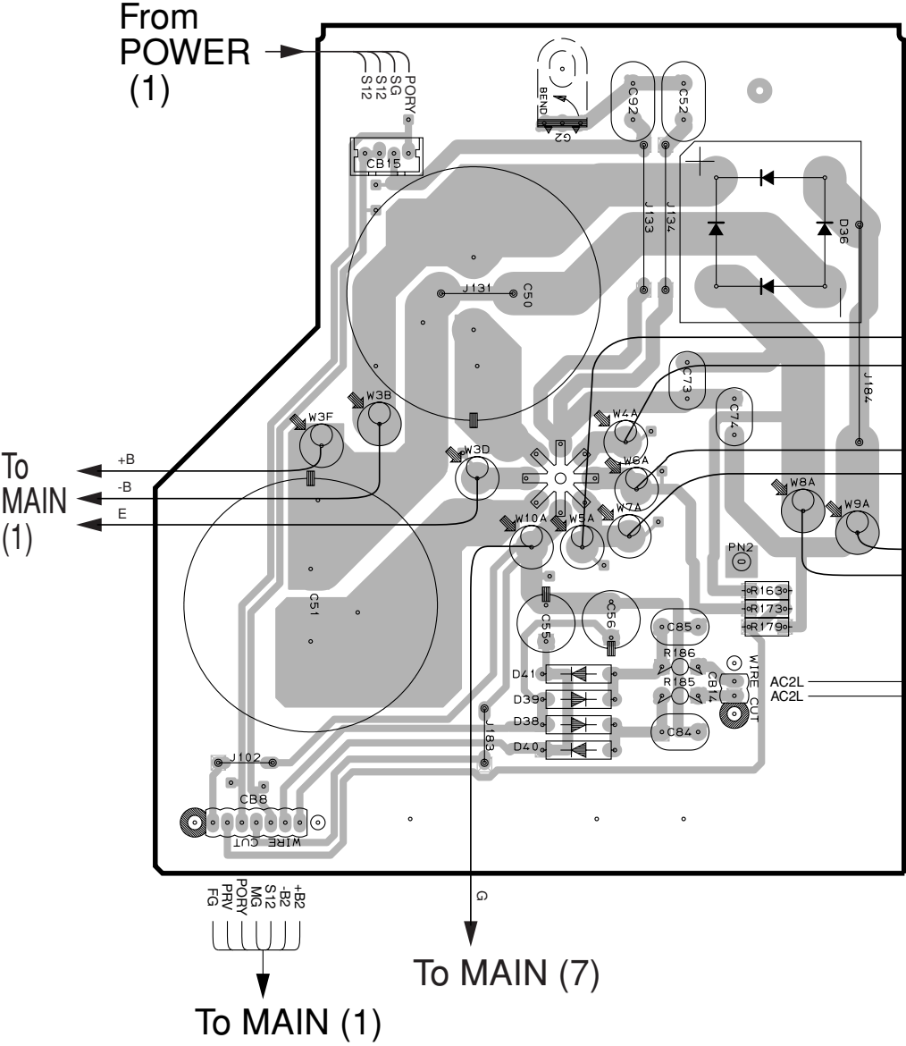
MAIN (3) P. C. B. (Lead Type Device)
