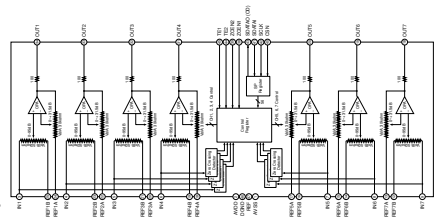
IC308; YAC523-EVR2 Digital volume
