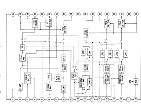
IC207: LA73654-TLME
