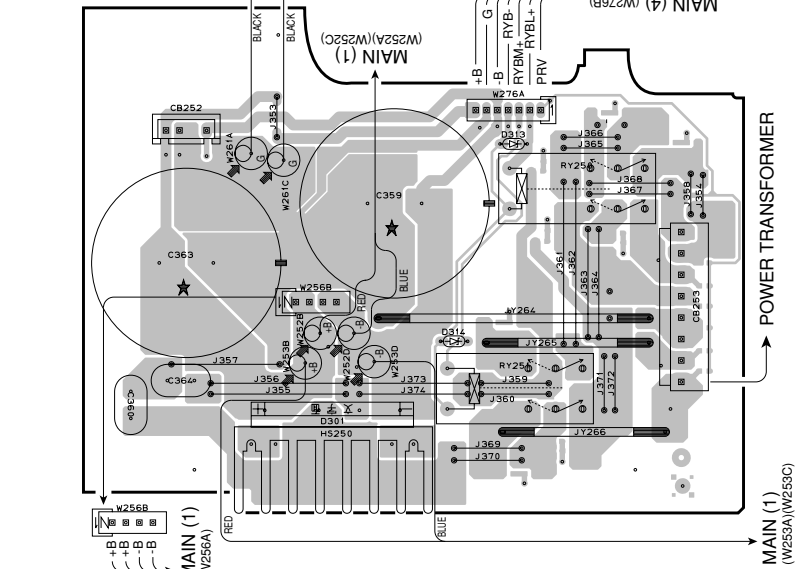
MAIN (2) P.C.B. (Side A)
