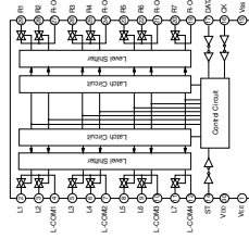
IC301: NJU731 1AM Analog function switch
